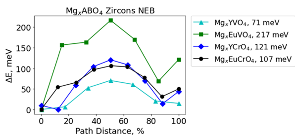
Figure 5. Energy profiles determined by DFT-NEB for \text{Mg}^{2+} migration across the characteristic \sim 1.5 Å linear hop at the dilute lattice limit (single Mg-ion in supercell) for zircon \text{YVO}_4 , \text{EuVO}_4 , \text{YCrO}_4 , and \text{EuCrO}_4 .
