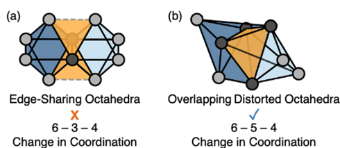
Figure 1. Visual representation of the characteristic structural motifs along diffusion pathways where the gray circles represent anions. Neighboring octahedral sites are colored with different shades of blue, while the intermediate tetrahedral sites are colored yellow. The darker gray-colored circles indicate which anions are shared by both octahedra. Panel (a) shows the edge-sharing octahedral motif found in previously studied cathodes (e.g., spinels, layered structures, and olivines) where there is no shared volume with the intermediate tetrahedral site. Panel (b) shows the overlapping distorted octahedral motif characteristic of zircon where volume is shared with the intermediate tetrahedral site.
