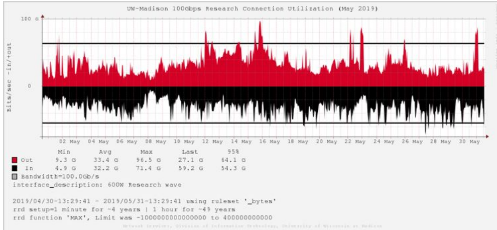
Figure 4 - UW 100Gbps research circuit utilization for May 2019.
