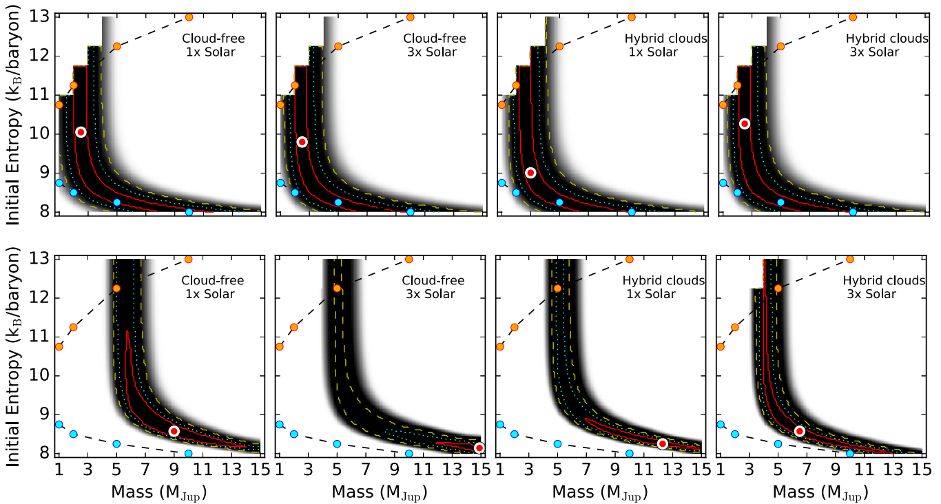
Figure 17. Comparison of the planet spectrum and luminosity to a combination of initial entropy ( k_B/\text{baryon} ) and planet mass ( M_{\text{Jup}} ) from the warm-start evolutionary models of Spiegel & Burrows (2012). The four different atmospheres tested include cloud-free and hybrid cloud models, with both solar and supersolar metallicity. Also plotted are the 1\sigma (solid red), 2\sigma (dotted cyan), and 3\sigma (dashed yellow) contours. The entropy plotted in the figure and used in the modeling is not the entropy for the evolved object but rather the entropy at formation. The best-fitting model fit is indicated by the large circle (white and red circle). The orange filled circles show the hot-start model limits, while the blue filled circles show the cold-start limits, which are presented as the boundary cases in Spiegel & Burrows (2012). The top row compares the model luminosity to the inferred luminosity for 51 Eri b, and the bottom row compares directly the SED to the evolutionary model spectra.
