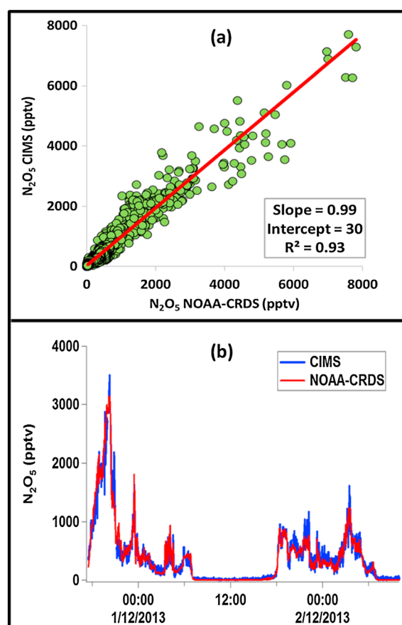
Figure 2. (a) Scatterplot between 1 min averaged \text{N}_2\text{O}_5 mixing ratios from the NOAA-CRDS (x axis) and from the CIMS (y axis) for 12 days ( N = 9148 ). Solid line (red) represents a RMA linear fit and (b) an example of \text{N}_2\text{O}_5 mixing ratios from CIMS and CRDS during nighttime and daytime.
