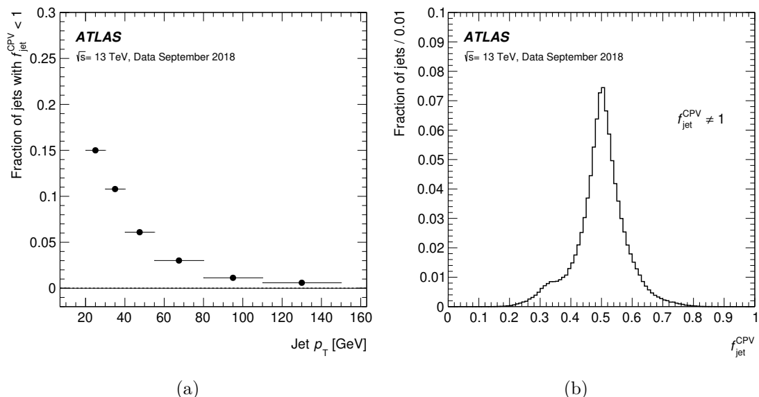
Figure 6. (a) Fraction of jets reconstructed from overlapping high-momentum signals in the detector, and (b) distribution of the jet overlap p_T fraction, f_{jet}^{CPV} , after removing the peak at f_{jet}^{CPV} = 1 containing 88% of selected jets. The pile-up dataset from a single ATLAS run taken in September 2018 is used, while a minimal selection of at least two jets with p_T > 20 GeV and satisfying the JVT requirement is applied. Statistical uncertainties are included, and are negligible.
