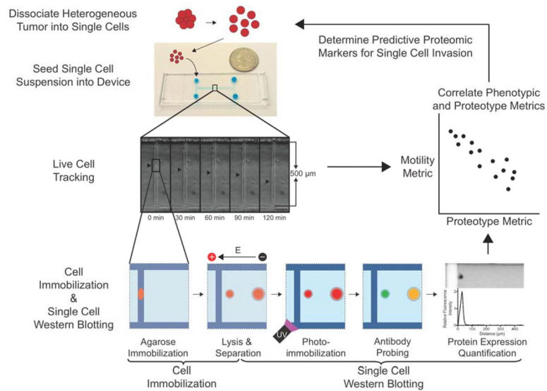
Figure 1. SCAMPR assay correlates cell migratory phenotype and protein expression. Microfluidic integration supports a Single-Cell Analysis of Motility and Proteotype (SCAMPR) assay. A heterogeneous population of primary cells is first dissociated into a single-cell suspension. The cells are then seeded into the SCAMPR device and tracked as each cell chemotactically migrates through the channels under a chemokine gradient, which reports motility and motility-related parameters, persistence and average aspect ratio. Immediately following the live-cell tracking, cells are immobilized in an agarose layer and the scWB is run in order to measure protein expression on each tracked cells. Motility and proteotype information from single cells is then correlated to associate proteomic markers with invasive motility properties.
