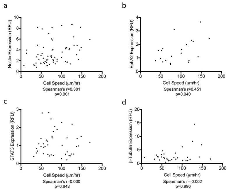
Figure 6. SCAMPR assay reveals Nestin and EphA2 correlate with TIC speed. Scatter plots of individual TICs show that (a) Nestin and (b) EphA2 are positively correlated with TIC speed (Spearman's rank r_{\text{Nestin}}=0.381 , p=0.001 , n=68 cells; r_{\text{EphA2}}=0.451 , p=0.040 , n=21 cells). However, (c) STAT3 and (d) \beta -tubulin are not correlated with TIC speed (Spearman's rank r_{\text{STAT3}}=0.030 , p=0.848 , n=43 cells; r_{\beta\text{-tubulin}}=-0.002 , p=0.990 , n=34 cells).
