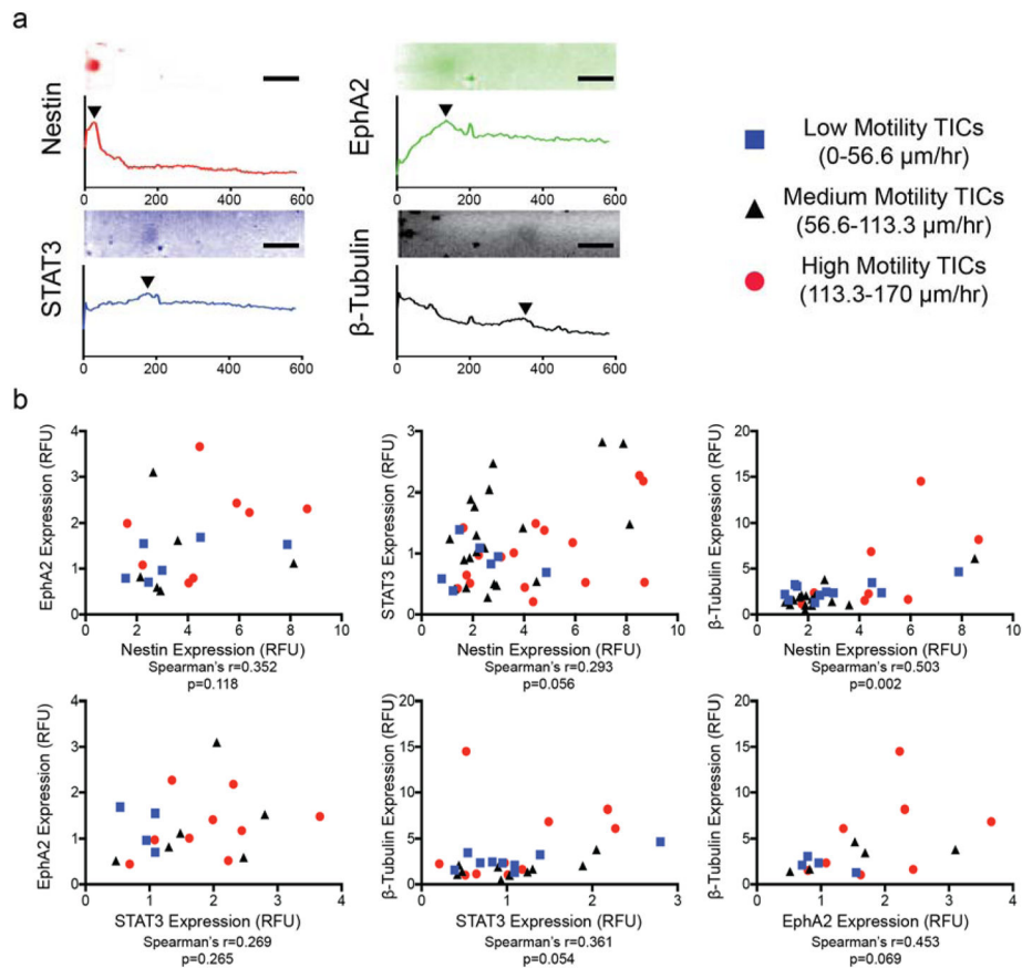
Figure 5. SCAMPR assay reveals novel protein expression correlations in GBM TICs. a) Representative fluorescence micrographs and intensity plots from the SCAMPR assay of GBM TICs. Arrows indicate peak location. Scale bars represent 100 μm. b) Biaxial scatter plots report protein expression for all markers for each GBM TICs from low, medium and high motility TIC subpopulations. Motility subpopulations were created based on three equally sized intervals of speed ranging from 0 μm per hr to 170 μm per hr (maximum observed TIC speed). TICs were binned into motility subpopulations based on magnitude of speed (Low Motility: 0–56.6 μm per hr, Medium Motility: 56.6–113.3 μm per hr, High Motility: 113.3–170 μm per hr). Blue squares, black triangles and red circles represent low, medium and high motility subpopulations, respectively.
