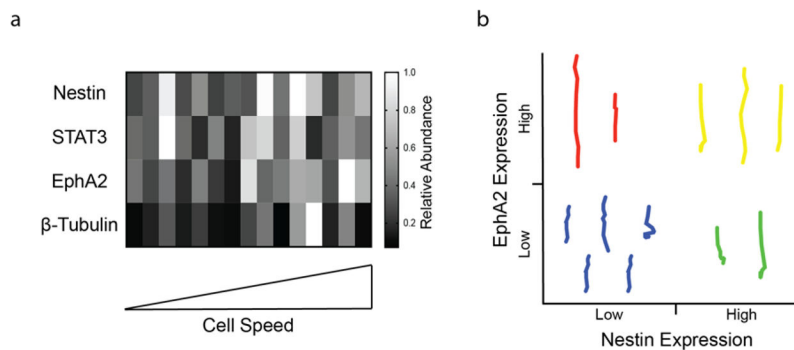
Figure 7. SCAMPR assay allows for joint multivariable analysis of phenotype and proteotype. a) Relative expression levels of Nestin, EphA2, STAT3, and \beta -tubulin in single GBM TICs with respect to cell speed. Only the subset of TICs with quantifiable expression levels for all four proteins is displayed in this plot. Protein expression in each TIC is normalized to the strongest signal for each protein. Within each row, tile color corresponds to relative expression level with black being the lowest and white being the highest. Each column represents the proteotype for one TIC and the TICs are organized in increasing cell speed order. b) Representative cell trajectories of single TICs expressing either low or high Nestin or EphA2. High and Low expression levels represent the top 50% and bottom 50% expression level for each respective protein.
