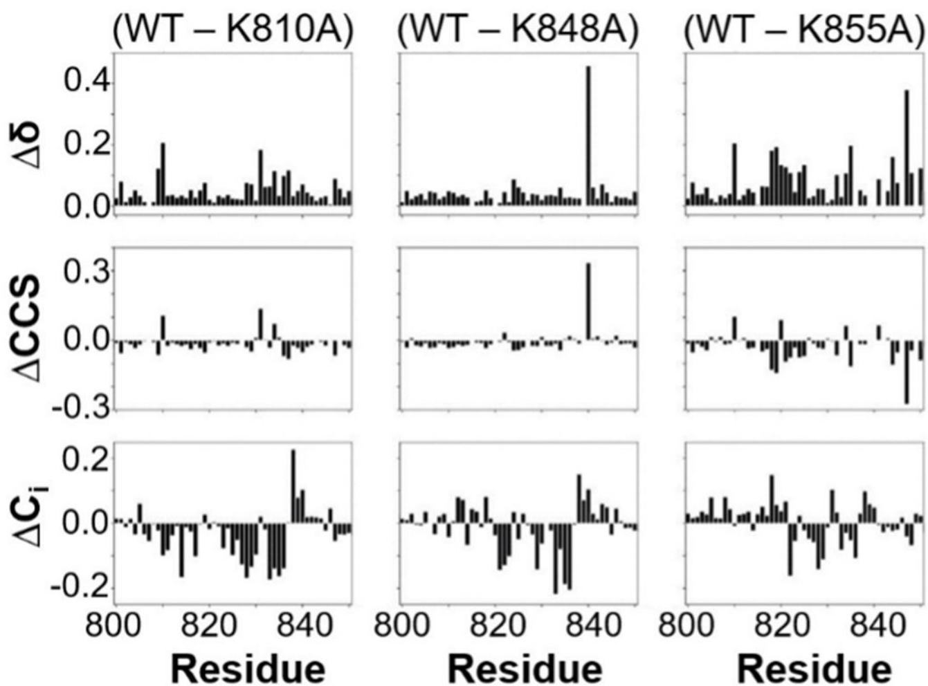
Figure 3. Relationship between the observed changes of chemical shift and the calculated difference in eigenvector centrality between wt and mutants K810A, K848A, and K855A. NMR-derived chemical shift perturbation ( \delta ), change in simulated composite chemical shift ( CCS ), and difference in eigenvector centrality derived from Kabsch-Sander hydrogen bond energy ( C_i ) between WT and mutants K810A, K848A, and K855A. Residues P800-D850 are shown. See Figure S2 and S3 for additional analysis.
