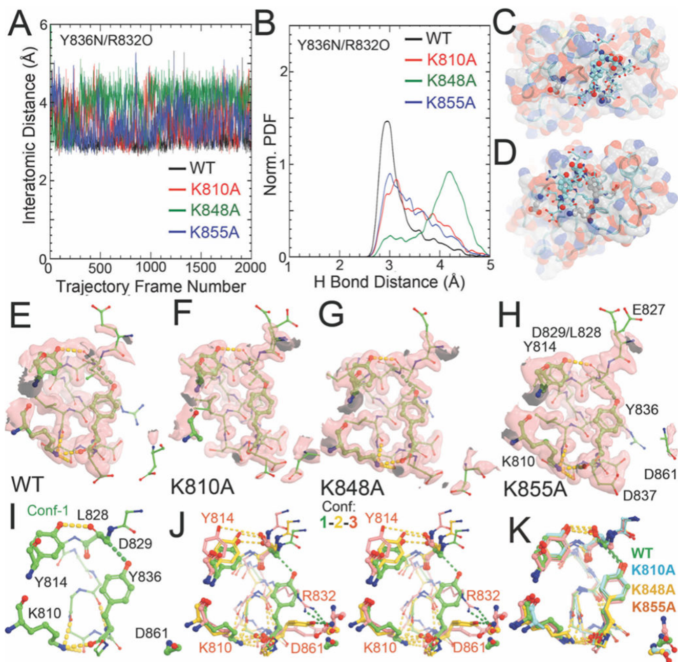
Figure 9. The structures of the Y836-containing loop in the wt enzyme and the three mutants. (A) Interatomic intra-loop Y836N-R832O distance as a function of MD trajectory frame for the wt enzyme (black), the K810A (red), K848A (green), and K855A (blue) mutants. (B) Corresponding relative PDFs. (C, D) Two views of the location of the Y836-containing loop within the HNH domain. (E-H). The Y836 loop-aligned MD-ED maps contoured at +6σ (isosurface) for the wt enzyme (E), the K810A (F), K848A (G), and K855A (H) mutants. (I) Two inter-loop H bonds (Y814O η /L828O, K810N ζ /Y836 and S834 and L833) and one intra-loop H bond (Y836N/R832O). (J) Stereodiagram of the Y836 loop in three
