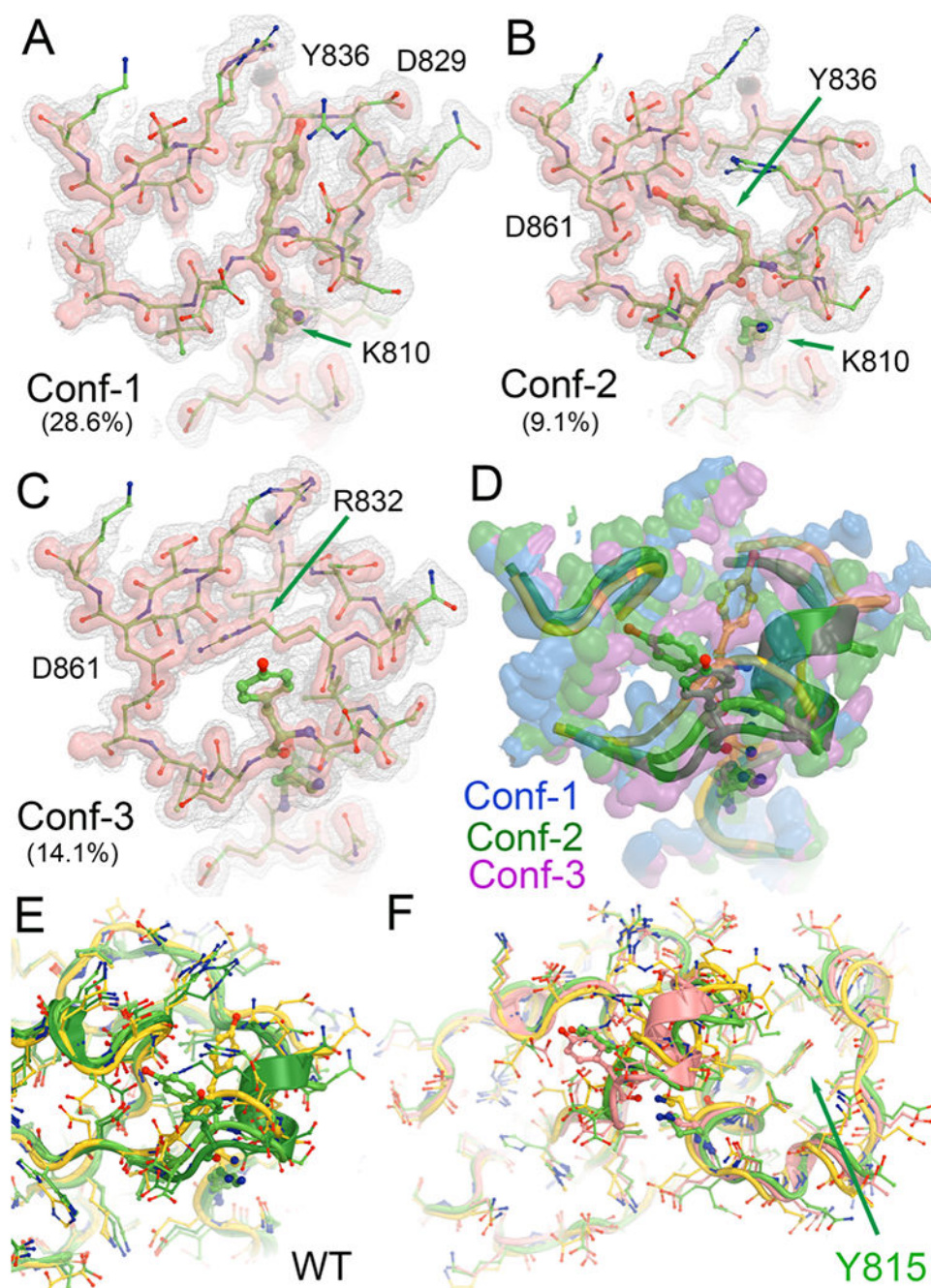
Figure 8. Decomposition of the three conformations of the wt enzyme through clustering analysis. (A) Conformation 1 (28.6%) at a low ( 2\sigma , silver isomesh) and high ( 6\sigma , salmon isomesh) contouring level superimposed with the corresponding equilibrated structure. (B) Conformation 2 (9.1%). (C) Conformation 3 (14.1%). (D) Superimposition of three conformations as unit population. (E, F) Two views of superposition of equilibrated structures corresponding to the three conformations.
