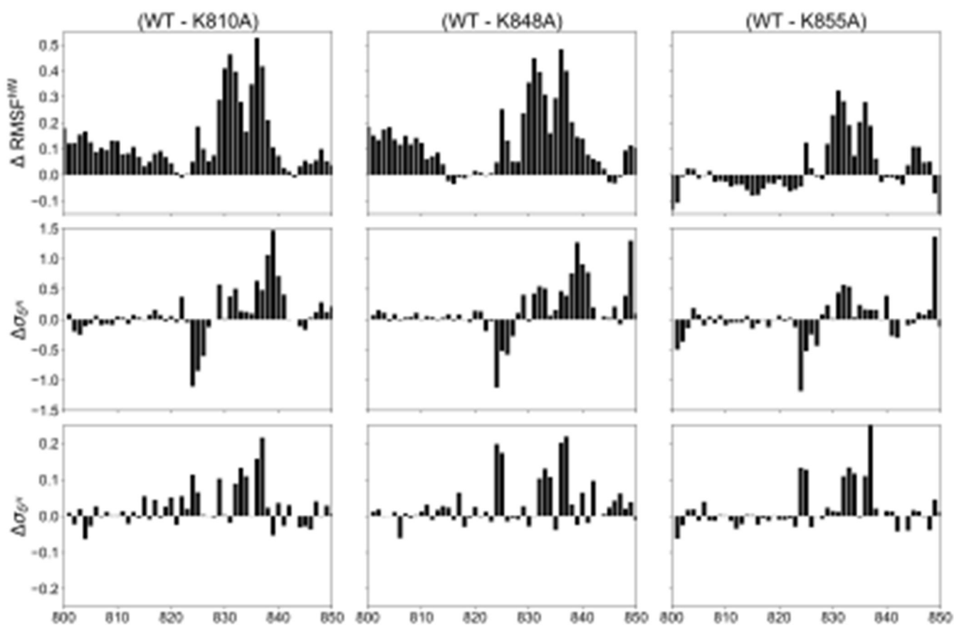
Figure 2. Apparent correlations of differences in RMSF values between the wt and each of the three mutants in the MD simulations with the simulated changes of NMR chemical shifts in residue range of P800-D850. See Figure S2 for additional analysis
