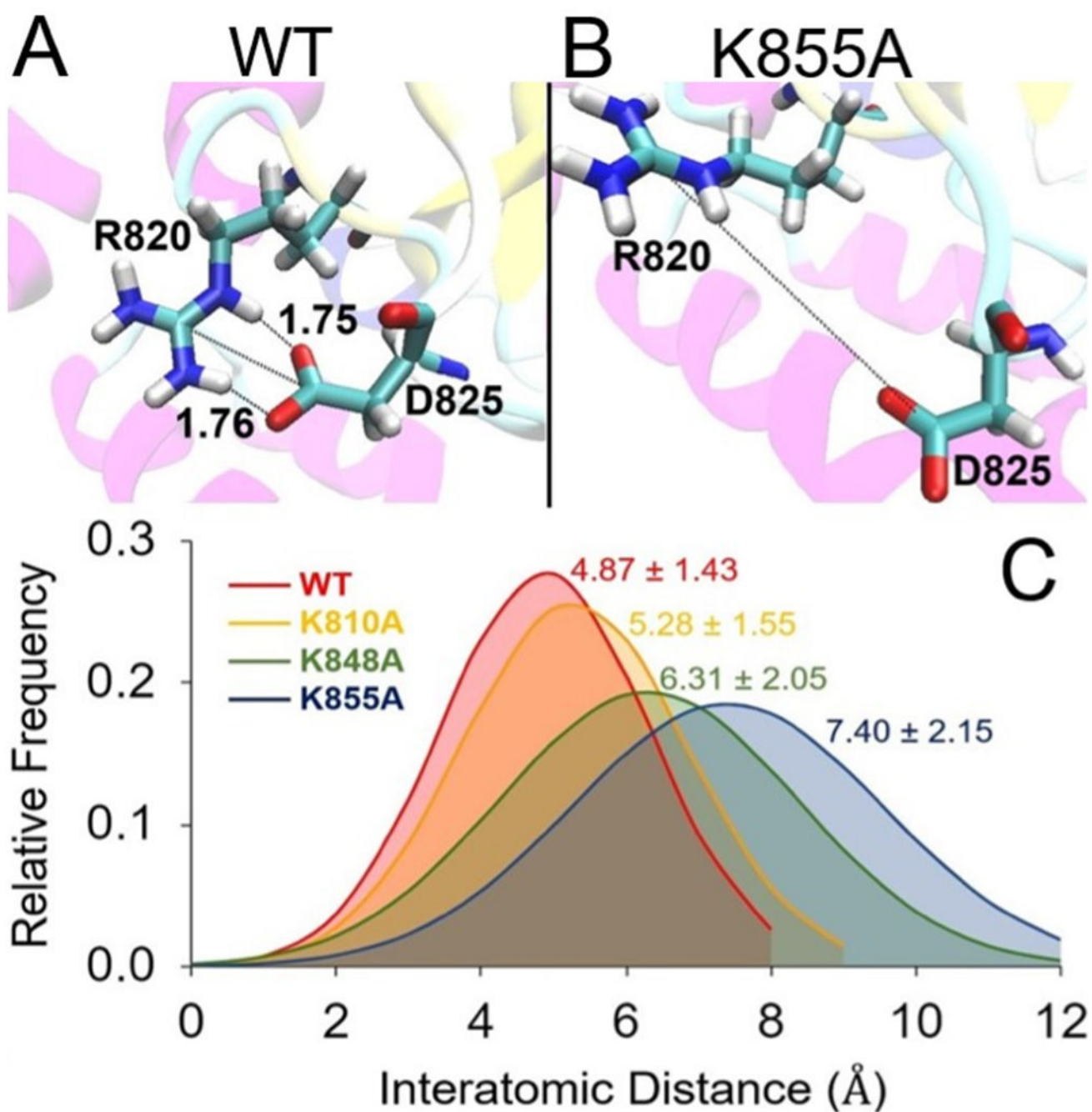
Figure 4. Close-up view of residues R820 and D825 (frame 526 of trajectory) in the HNH domain. (A) wt: two hydrogen bonds are detected (1.75 Å and 1.76 Å). (B) In the K855A mutant, both H-bonds disappear. (C) Relative distance probability density function as a function of interatomic R820-D825 distance for the wt (red), K810A (orange), K848A (green), and K855A (blue) mutants. See Figure S4 for additional analysis.
