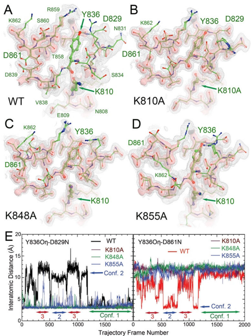
Figure 6. MD-derived ED maps for the wt (A), K810A (B), K848A (C) and K855A (D) mutants at a low ( 2\sigma , silver isomesh) and high ( 6\sigma , salmon isomesh) contouring level superimposed with the corresponding MD ESP map-derived equilibrated structures. (E) Interatomic Y836O \eta -D829N distance for conformation 1 (left) as a function of MD trajectory frame number for wt (black), the K810A (maroon), K848A (green), and K855A (blue) mutants. Interatomic Y836O \gamma -D861N distance (right) for clustering the second conformation of the
