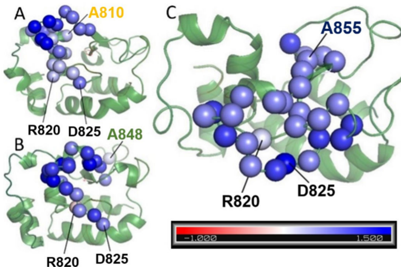
Figure 5. Difference in eigenvector centrality between wt and (A) K810A, (B) K848A, and (C) K855A mutants with \lambda (locality factor) of 20 Å. Residues with differences in eigenvector centralities greater than 2 standard deviations from the mean are represented as spheres and colored according to the color bar (dominated by large values in blue). In addition to given Lys-to-Ala mutations, the locations of R820 and D825 are also indicated.
