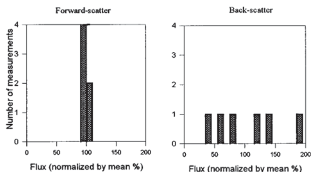
Fig. 6 Measurement results at six different testing points using (a) FSD and (b) BSD at a set flow rate of 0.5 ml/min.
