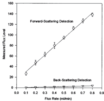
Fig. 4 Typical measurements obtained from FSD and BSD at testing point 5 on the tooth.
