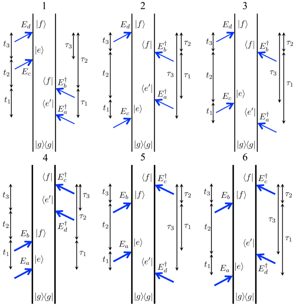
Figure 2. (Color online) Ladder diagrams for the TPA signal with selected phase e^{i(\phi_a + \phi_b - \phi_c - \phi_d)} . Both loop \tau_j and ladder t_j delays, j = 1, 2, 3 are indicated. The transformation between two is different for each diagram. Time translation invariance implies \omega + \omega_b - \omega_c - \omega_d = 0 . The LOP signal is a sum of all six diagrams whereas the LAP can be separated into k_I , k_{II} and k_{III} signals (see text).
