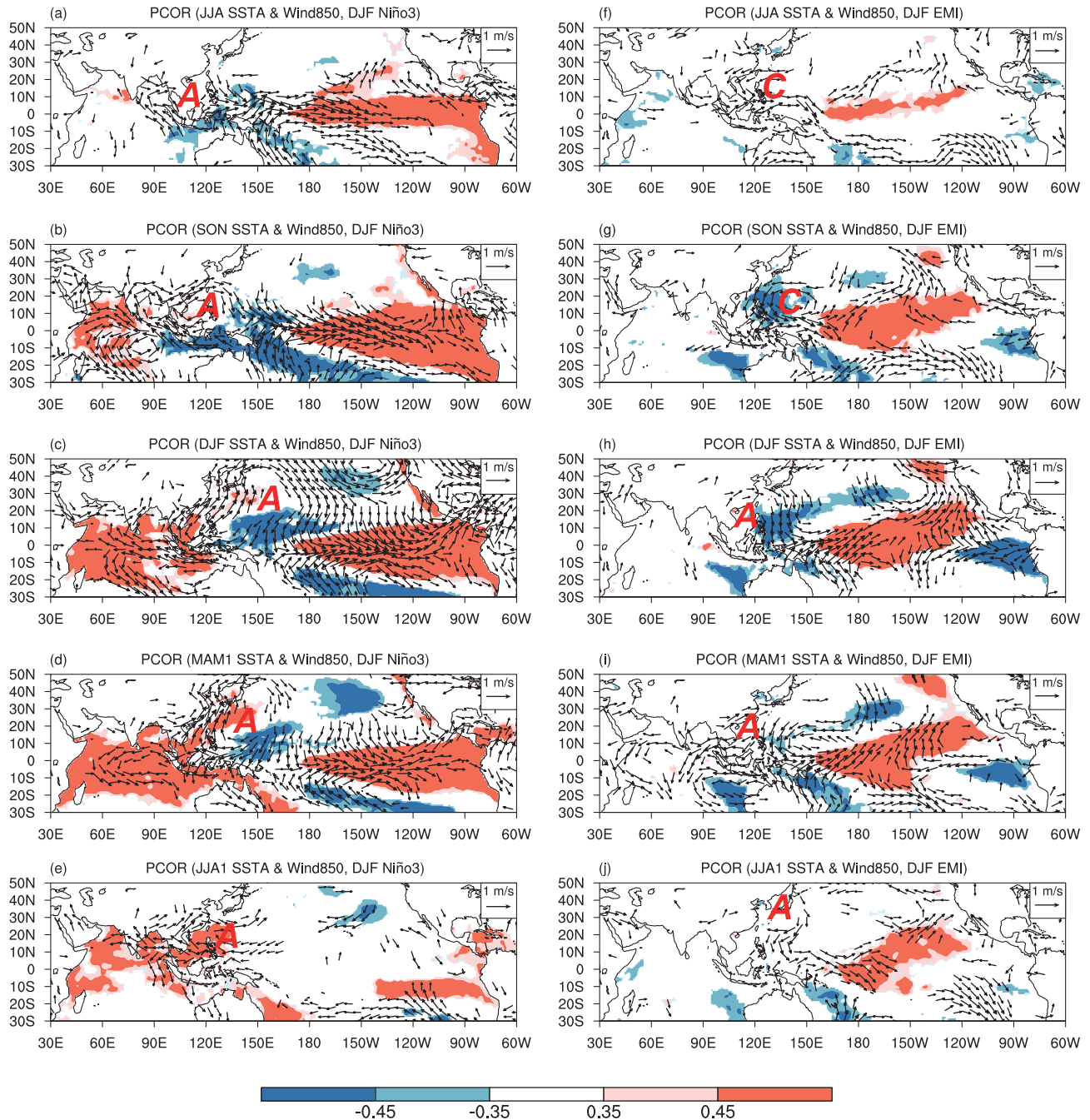
Figure 4. (a)–(e) Partial correlations of seasonal SST (shadings) and 850-hPa winds (vectors) with normalized DJF Niño-3 indices and (f)–(j) DJF EMI (El Niño Modoki) indices. Shadings indicate correlations above the 95% and 99% confidence levels; only the vectors significantly above the 95% confidence level are shown. ‘C’ (‘A’) denotes anomalous cyclone (anticyclone) (from fig. 1 in Yuan et al. [151]).
