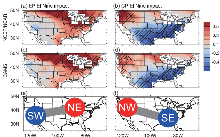
Figure 3. US winter (JFM) surface air temperature anomalies regressed onto EP El Niño (left panels) and CP El Niño (right panels) indices based on (a) and (b) the NCEP-NCAR reanalysis and (c) and (d) the CAMS air temperature data set. Regression coefficients significant at the 90% confidence level are shaded. (e) and (f) Conceptual diagrams of the impacts of EP El Niño and CP El Niño on US winter surface air temperature (from fig. 1 in Yu et al. [30]).
