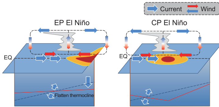
Figure 1. Conceptual diagram for the spatial patterns of EP El Niño events (left figure) and CP El Niño events (right figure). Arrows with (without) white borderlines represent anomalous oceanic (atmospheric) circulations, respectively. Shadings at the sea surface denote the spatial location of the SST anomaly. Dashed blue lines and solid red lines represent the climatological and El Niño-conditioned equatorial thermocline, respectively (adapted from fig. 3 in Yeh et al. [54]).
