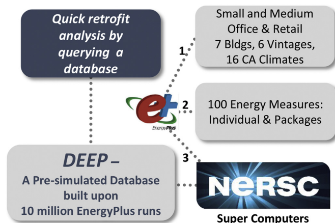
Fig. 1. Overview of DEEP.
