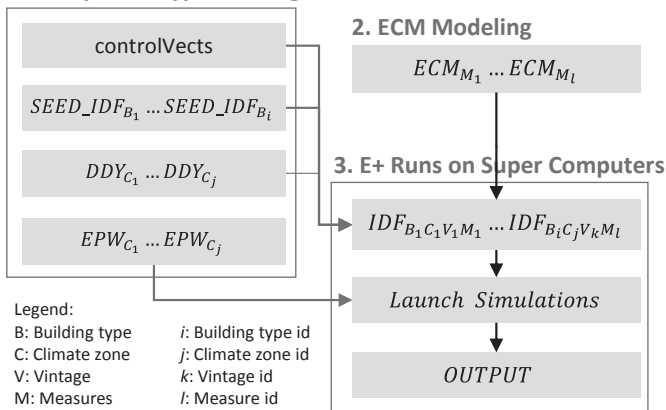
Fig. 3. The framework used for establishing DEEP.
