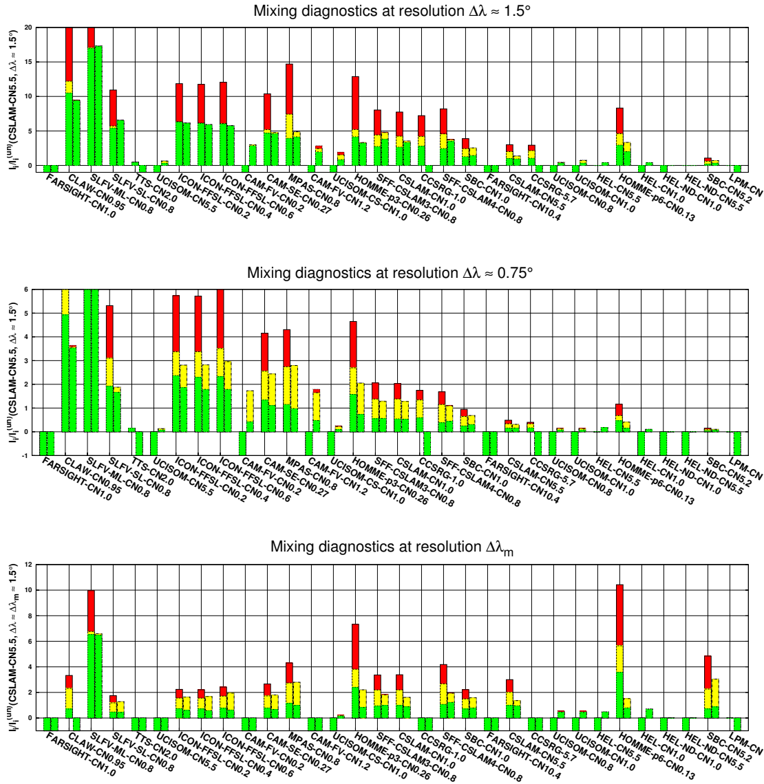
Fig. 15. A histogram of mixing diagnostics (stacked) at resolutions \Delta\lambda \approx 1.5^\circ (upper), \Delta\lambda \approx 0.75^\circ (middle), and \Delta\lambda \approx \Delta\lambda_m (lower). The ordering is according to minimal resolution \Delta\lambda_m for the respective unlimited schemes (see Fig. 3 first row). Above each scheme acronym there are two columns of data. The left column is for the unlimited scheme, and the right column contains data for the shape-preserving version of the scheme (if applicable). The height of each colored column (green \ell_r , yellow \ell_u , red \ell_o ) is the ratio between \ell_i , i \in \{“r”, “u”, “o”\} for the scheme in question normalized by the \ell_i for CSLAM (CN5.5) at \Delta\lambda = 1.5^\circ . Note that the y axis scale are different. The stacked histograms for SLFV-ML and CLAW exceed the plotting range. If no data are available, the mixing data are negative (although \ell_i data were not submitted for FARSIGHT, there are some mixing diagnostics given in White and Dongarra, 2011). The numerical values for \ell_i are listed in the scatterplots in Figs. 11, 12, 13 and 14.
