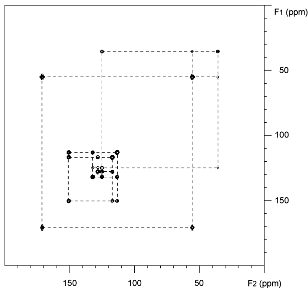
Fig. 5. The ^{13}\text{C} UC2QF COSY of U- ^{13}\text{C} , ^{15}\text{N} tyrosine (diluted to 50% in unlabeled tyrosine). Data were acquired on a 9.4 T Bruker DSX spectrometer ( ^1\text{H} frequency 400.13 MHz) equipped with a double-resonance 2.5 mm MAS probe spinning at 30 kHz. The pulse sequence from Fig. 2A was used with the preparatory pulse replaced by cross-polarization from protons. 50 kHz ^{13}\text{C} pulses were used throughout, along with 80 kHz TPPM ^1\text{H} decoupling. The full phase cycle of Table 1 was used. Two hundred and fifty six points were acquired with a spectral width of 25 kHz in t_1 and 1024 points were acquired in t_2 with a spectral width of 25 kHz.
