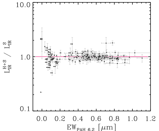
Fig. 5 Ratio of the total IR luminosity ( L_{\text{IR}} ) estimated using both Herschel and Spitzer data ( L_{\text{IR}}^{\text{H+S}} ) over the one using only Spitzer ( L_{\text{IR}}^{\text{S}} , see Wu et al. 2010) as a function of the EW_{6.2} . (see Section 3.3). The solid purple line corresponds to the 1-to-1 relation between the two L_{\text{IR}} estimates.
