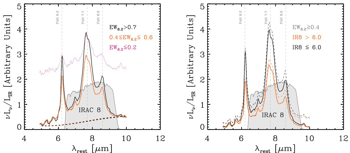
Fig. 9 Left : Average spectra in various EW_{6.2} bins in the 4 - 10\ \mu\text{m} range. The dashed lines correspond to the underlying continuum emission as inferred by PAHFIT. The grey shadowed area depicts the 8.0\ \mu\text{m} IRAC filter. Right : Average (dashed lines), and average continuum subtracted (solid lines) spectra of all galaxies with EW_{6.2} \geq 0.4\ \mu\text{m} grouped in those with IR8 > 6 (orange lines), and IR8 < 6 (black lines)
