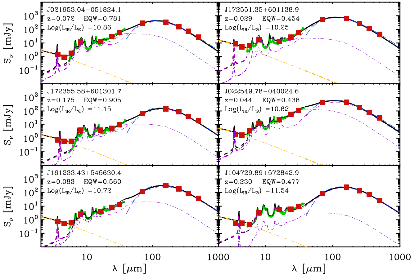
Fig. 3 Examples of SED fitting. Red squares are observed points, overlaid with the best-fit DL07 model (black line). The PDR and diffuse ISM components are shown in purple. The yellow line is the stellar component and the dashed blue line the best-fit modified blackbody model with \beta = 1.5 . The green line in the mid-IR is the actual IRS spectrum of each source. We convolved the observed IRS spectrum with the IRS 16\mu\text{m} peak-up imaging filter and a 2\mu\text{m} -wide top-hat filter centred at observed 30\mu\text{m} to enhance our fit with two more points in the observed mid-IR part of the spectrum. The rest of the data are taken from IRAC, MIPS, and SPIRE.
