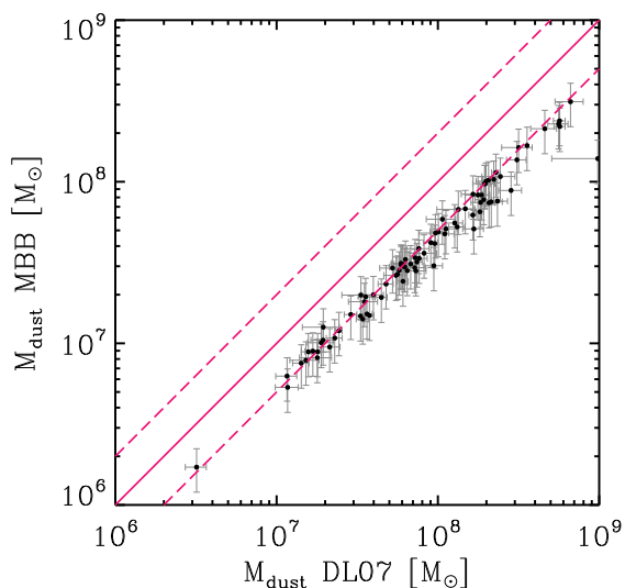
Fig. 4 Comparison between dust masses derived based on a single-temperature modified blackbody (MBB) and masses derived using the Draine & Li (2007) models. For the MBB derived M_{\text{dust}} we assume \beta = 1.5 . The purple solid line corresponds to unity and the two purple dashed lines to its offset by a factor of 2 and 0.5.
