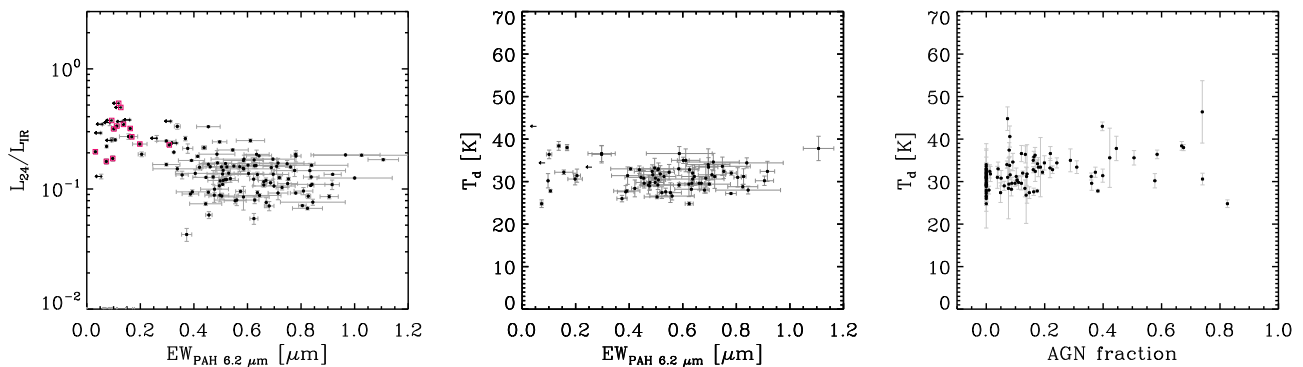
Fig. 6 Left: L_{24} / L_{\text{IR}} ratio as a function of the 6.2 \mu\text{m} PAH feature EW. Purple squares correspond to sources for which the SED decomposition suggests that the AGN contribution to the total L_{\text{IR}} is > 50\% . Leftward arrows denote upper limits in EW_{6.2} measurements. Middle: T_d versus EW_{6.2} . T_d estimates are derived based on a modified blackbody model for 79 sources (out of the total 154 sources shown in the left panel), which are detected in at least three bands at \lambda_{\text{rest}} > 60 \mu\text{m} . Right: T_d versus fraction of L_{\text{IR}} arising from AGN activity, as derived based on SED decomposition.
