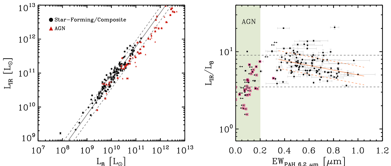
Fig. 8 Left : L_{\text{IR}} versus L_8 for the whole 5MUSES sample. Black circles correspond to purely star-forming and composite sources, while red triangles correspond to AGN. The solid grey line depicts the median and 68% dispersion of composite and star-forming galaxies. Right : L_{\text{IR}}/L_8 versus EW of 6.2\ \mu\text{m} . The horizontal lines enclose the values of L_{\text{IR}}/L_8 within the 68% dispersion from the median. The orange lines depict the best-fit linear regression and its scatter in the EW_{6.2} \geq 0.4\ \mu\text{m} regime. Purple squares correspond to sources with f_{\text{AGN}} > 0.5 .
