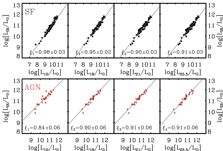
Fig. 11 Correlation between L_{\text{IR}} and rest-frame luminosities at observed 10, 18, 21-, and 25.5 \mu\text{m} . The choice of the rest-frame luminosity wavelengths corresponds to the central wavelengths of the JWST-MIRI filters. Each IRS spectrum was shifted to the rest-frame and convolved with MIRI filters. The best-fit regression line and the associated plot are shown in each panel and are summarised in Table 3.
