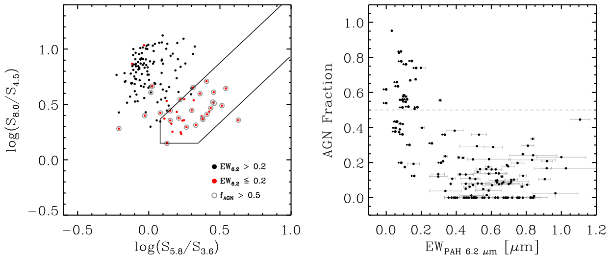
Fig. 1 Left : IRAC colour-colour diagram of the 5MUSES sample. The wedge is the AGN selection region of Donley et al. (2012). Red and black circles represent sources with EW_{6.2} \leq 0.2\ \mu m and EW_{6.2} > 0.2\ \mu m respectively. Grey circles correspond to sources for which the SED decomposition attributes more than 50% of their total infrared luminosity to AGN activity. Right : Fractional contribution of an AGN component to the total L_{IR} as a function of the 6.2\ \mu m EW of the sources. The dashed grey line corresponds to f_{AGN} = 0.5 .
