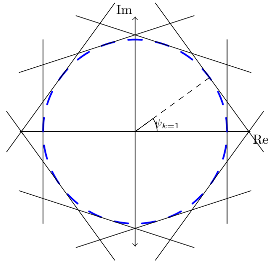
Figure 2.5: A constraint on apparent power approximated by linear half-spaces
