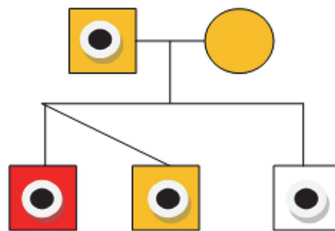
Fig 3. Coding variants observed in SLIC probands and their families. Pedigrees are shown for nuclear families of SLIC individuals carrying three coding variations in NFXL1 . Individuals carrying the variants are identified with a black circle. Sequencing traces of each variant is shown. SLIC probands are colored in red and other family members with SLI (defined as expressive and/or receptive language skills >1.5SD below that expected for their age) are colored in orange. In pedigree 3 (rs151113647), the youngest sibling (colored in yellow) did not meet the criteria for SLI but had expressive and receptive language scores ~1SD below that expected for his age. Individuals with no shading have typical language ability. DNA was not available for individuals colored in grey.
