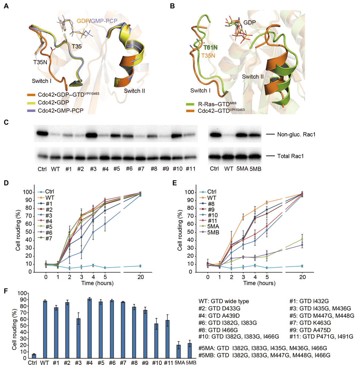
Fig. 3. GTD grips Rho/Ras mostly via their switch I and II regions, and these interactions are crucial for its cytopathic effect. (A) Superposition of the structures of the Cdc42-GDP-GTD VP110463 complex, Cdc42-GDP (PDB: 1ANO, yellow), and Cdc42-GMP-PCP ( \beta,\gamma -methyleneguanosine 5'-triphosphate) (PDB: 2QRZ, light blue) focusing on the switch I and II regions. GDP and GMP-PCP are shown as sticks. Residues T35 in the WT Cdc42 and T35N in the Cdc42-GDP-GTD complex are shown as sticks. (B) Structural comparison between the GTD M68 -bound R-Ras and the GTD VP110463 -bound Cdc42, focusing on the switch I and II regions. Residues T61N R-Ras and T35N Cdc42 are shown as sticks. (C) The glucosyltransferase activities of the selected GTD VP110463 mutants toward the recombinant Rac1 were examined using an in vitro assay. (D and E) The cytopathic effects of the GTD VP110463 mutants were examined using the cell-rounding assay, and the percentage of rounded cells was quantified. (F) The percentages of rounded cells at 5 hours after treatment. The data are presented as means \pm SD, n = 3 .
