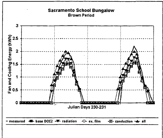
Figure 4. DOE2 simulation results for the Sacramento school bungalow in 1992 during Julian days 230 and 231, when the bungalow had a brown painted roof surface. Actual measured data are shown by the solid line. DOE2 results without the roof-attic function are shown, as well as results using the roof-attic function with only radiative exchange, only a lowered exterior film convection correlation, only enhanced insulation thermal conductivity with temperature, and with all radiative, convective and conductive changes.
