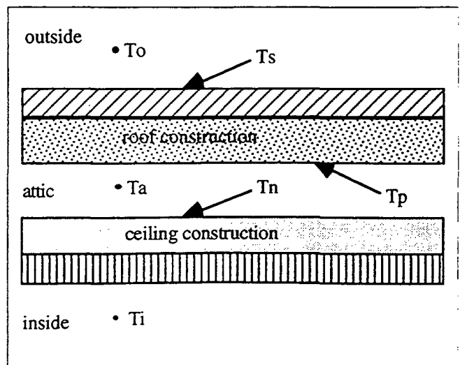
Figure 1. Designation of surface temperatures used in equations 1 through 4.
