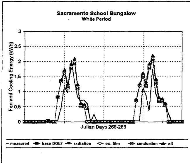
Figure 5. DOE2 simulation results for the Sacramento school bungalow in 1992 during Julian days 268 and 269, when the bungalow had a white painted roof surface. Actual measured data are shown by the solid line. DOE2 results without the roof-attic function are shown, as well as results using the roof-attic function with only radiative exchange, only a lowered exterior film convection correlation, only enhanced insulation thermal conductivity with temperature, and with all radiative, convective and conductive changes.
