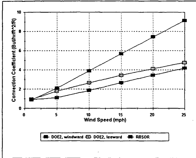
Figure 2. Comparison of external convection coefficients calculated by DOE2 and RBSOR models. Calculations were made for ambient temperature of 85°F, surface temperature of 130°F, and characteristic length of 30 feet on a horizontal surface. The convection coefficients used in the RBSOR model are about half the value of the DOE2 windward coefficients.
