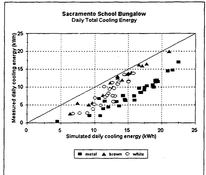
Figure 6. DOE2 simulated daily total cooling energy for the Sacramento school bungalow versus measured daily total cooling energy. The DOE2 simulation uses the roof-attic function with radiative, convective and conductive options in uses. Days with the metal, brown painted and white painted roof surfaces are identified with different symbols. The line from the bottom left corner to the top right corner represents the line where measured and simulated data are equal—the closer the data to this line, the better the simulation.
