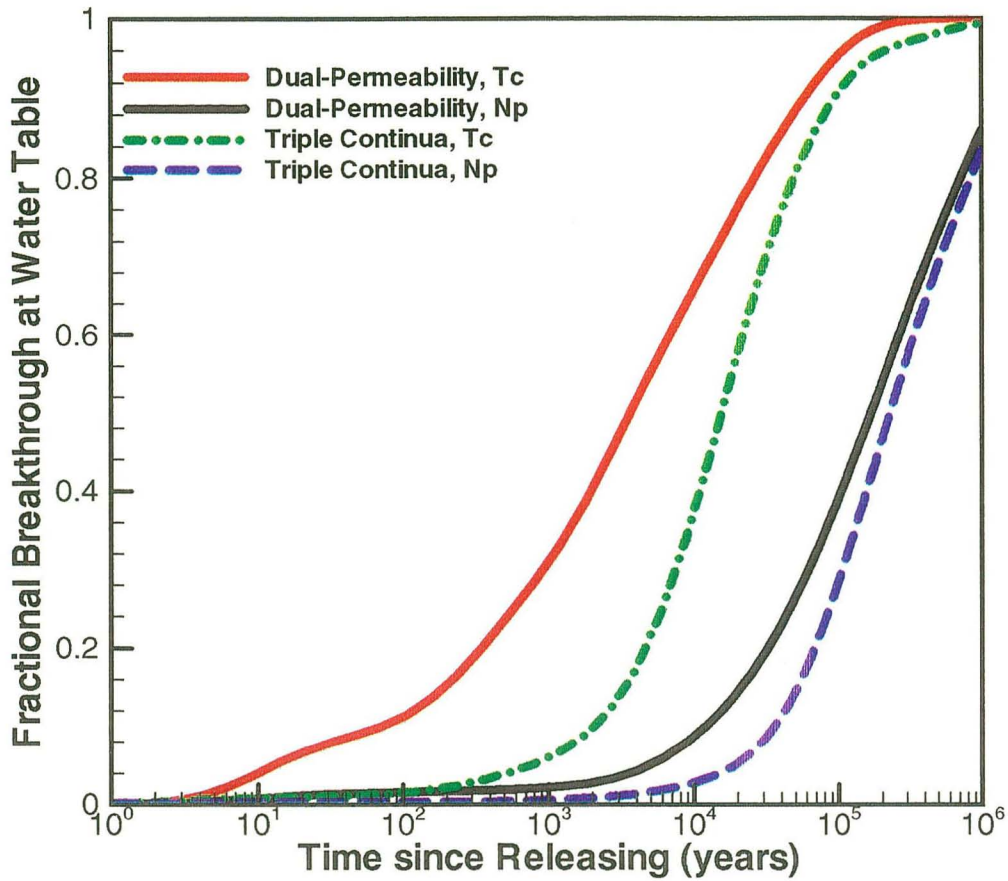
Figure 13. Comparison between cumulative breakthrough curves at the water table, simulated for conservative and reactive tracer transport from the repository with the dual-permeability and triple-continuum 3-D models, respectively.
