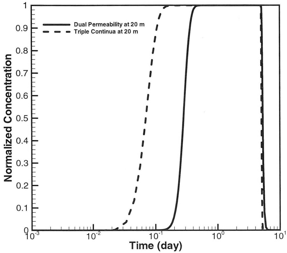
Figure 6. Breakthrough curves of relative tracer concentration at 20 m from the well for the scenario of dual-permeability model fracture porosity equal to combined porosity of large and small fractures in a triple-continuum model.
