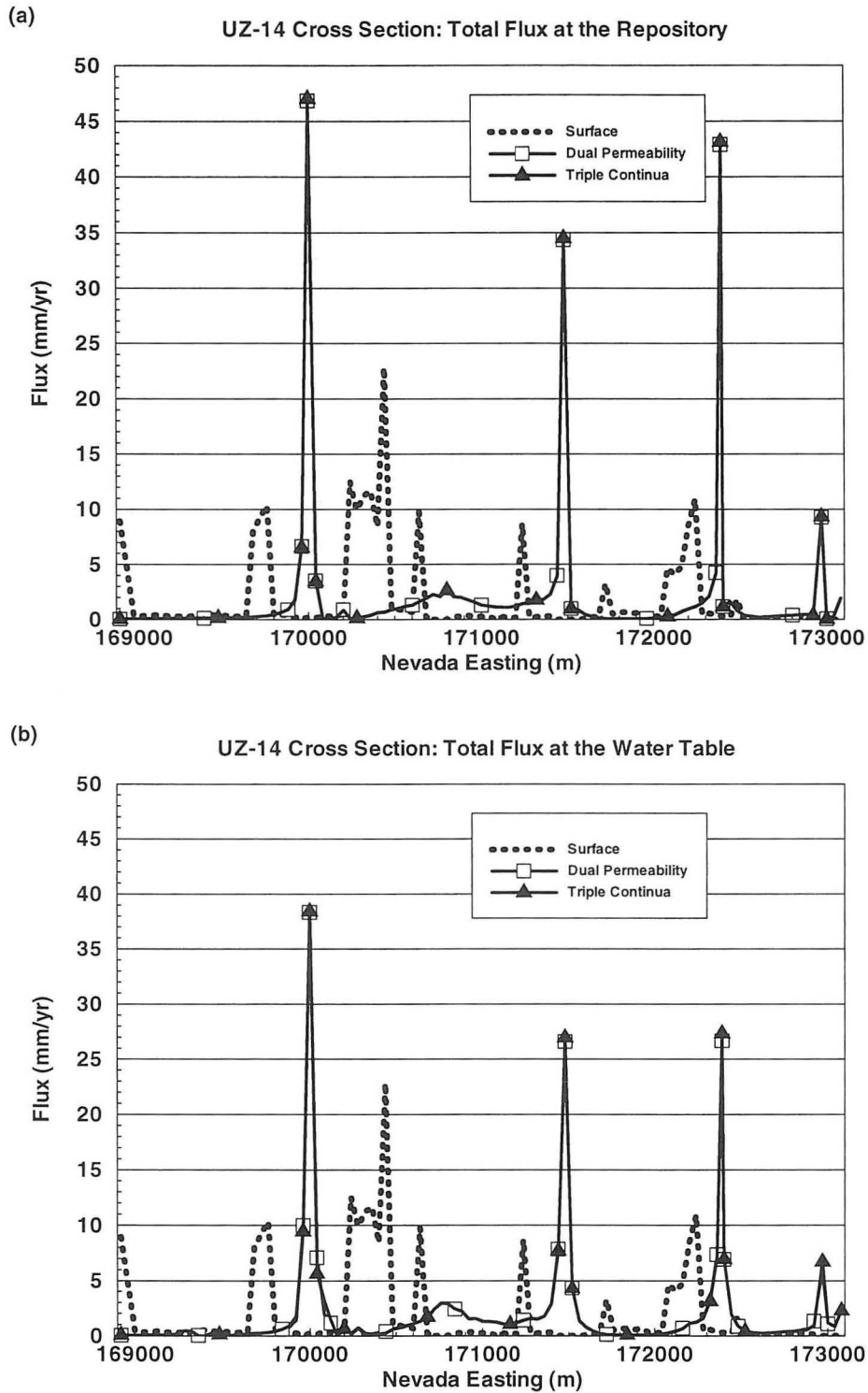
Figure 15. Comparison of surface infiltration rates and percolation fluxes (a) at the repository level and (b) at the water table, respectively, simulated using the dual-permeability and triple-continuum 3-D models.
