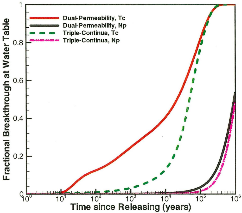
Figure 16. Comparison between cumulative breakthrough curves at the water table, simulated for conservative and reactive tracer transport from the repository, with the dual-permeability and triple-continuum 2-D models, respectively.
