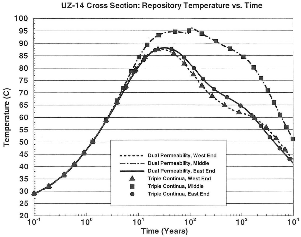
Figure 17. Comparison of repository temperature variations at three locations, simulated using the dual-permeability and triple-continuum 3-D models.
