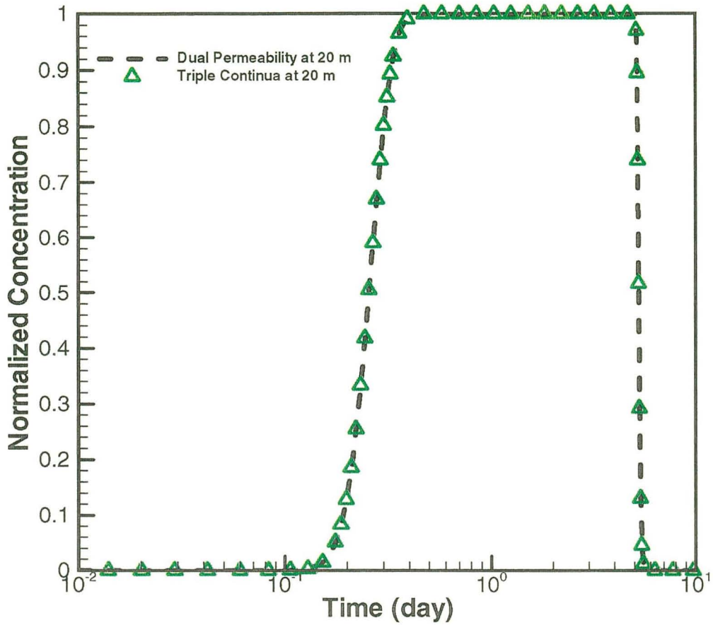
Figure 7. Breakthrough curves of relative tracer concentration at 20 m from the well for the scenario of dual-permeability model fracture porosity equal to large-fracture porosity with a triple-continuum model.
