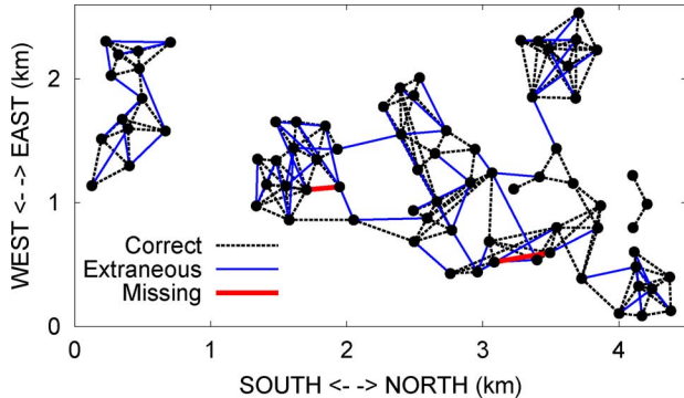
Fig. 6. Accuracy of an estimated conflict graph.
