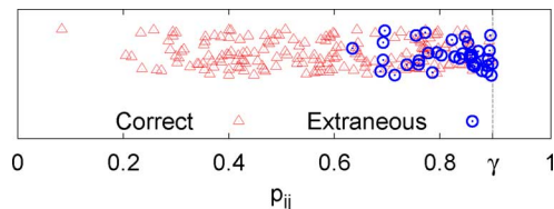
Fig. 8. Values of p_{ij} for both correct and extraneous edges in the estimated conflict graph, using the Street model and \gamma = 0.9 . We denote the two kinds of edges with different markers and spread them out vertically using random y values.
