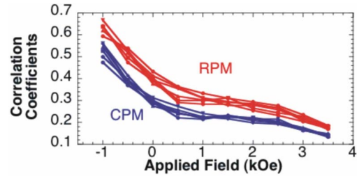
FIG. 3 (color online). Measured RPM and CPM values versus the applied field for the 8.5 milliTor sample.
