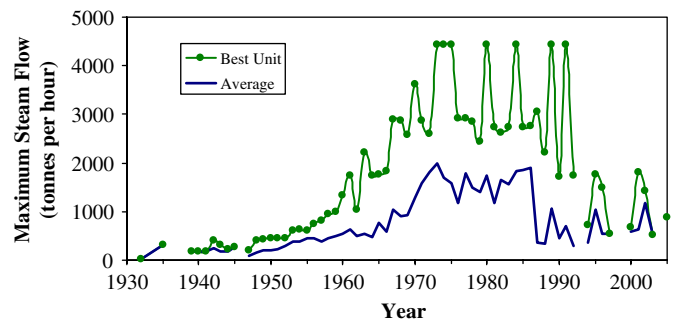
Fig. 7. Maximum continuous steam flow at 100% load (in thousands of pounds per hour) for coal-fired utility boilers. Source: [46].
