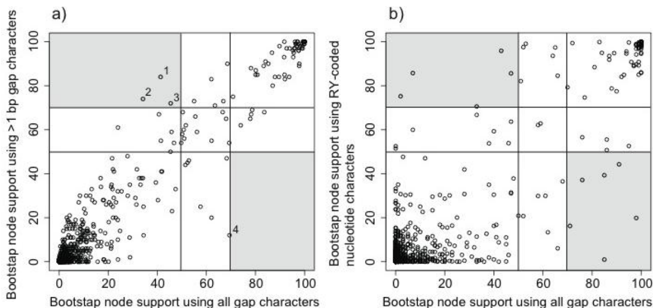
Figure 5. (a) Comparison of bootstrap support in trees based on all gap characters and gap characters >1-bp in length. Bipartitions that appeared well supported ( \geq 70\% bootstrap) by one analysis and poorly supported ( < 50\% bootstrap) in the other are shaded. Numbers correspond to the following bipartitions: 1. Ardea-Cochlearius-Eudocimus ; 2. Alisterus-Psittacula ; 3. Chalcopsitta-Platycercus ; and 4. Picodynastornites. (b) Comparison of bootstrap support for analyses using all gap characters and RY-coded nucleotide data. The same numbers of informative characters were used in each of these analyses (next page).
