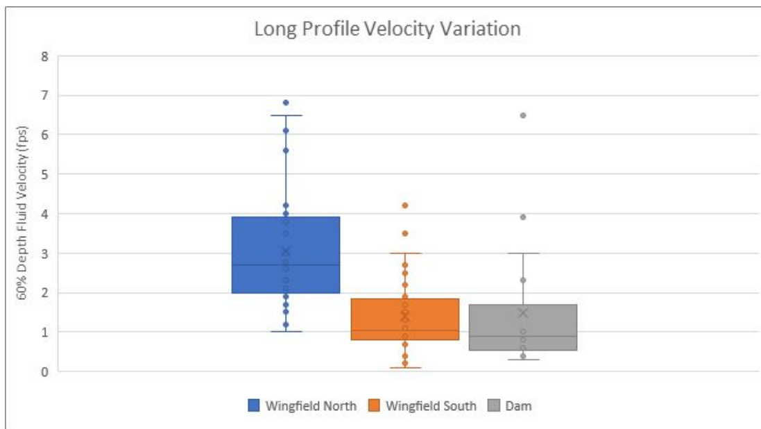
Figure 22: Velocity along the longitudinal profiles. Point velocities taken approx. every 15 ft.
