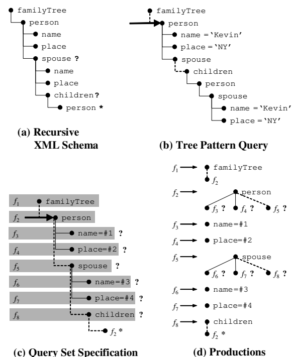
Figure 3 Family Tree Recursive Example
