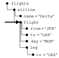
(b) Tree Pattern Query
