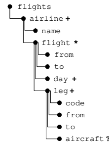
(a) Data XML Schema
