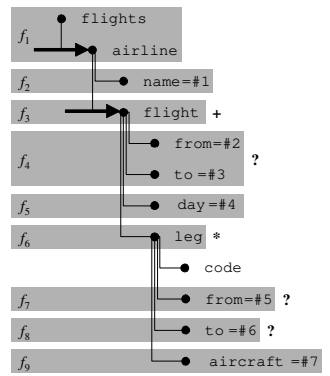
(c) Query Set Specification
