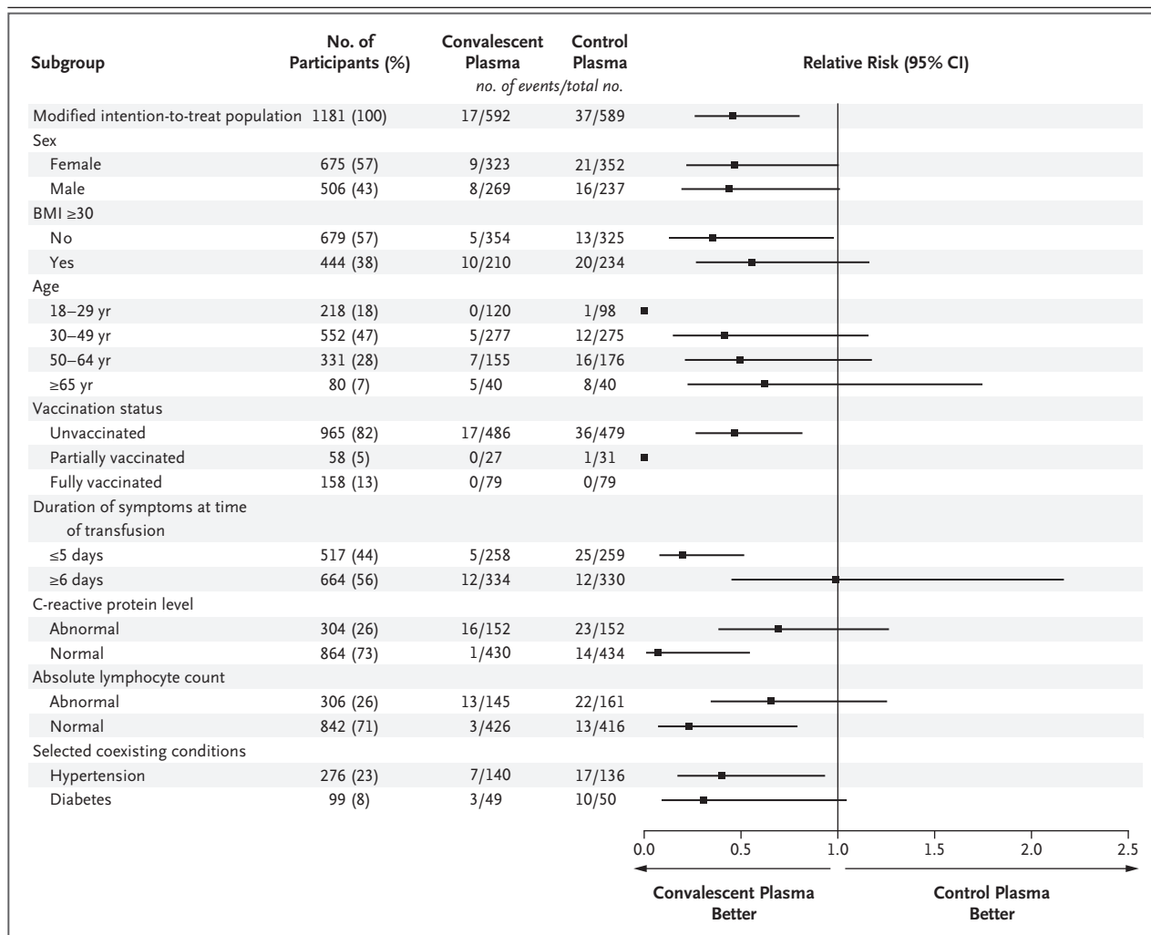
Figure 3. Subgroup Analyses.
