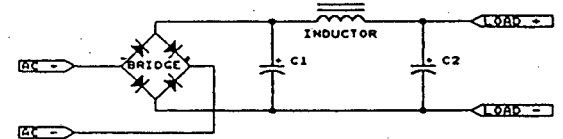
Figure 6. Passive power factor correction III.
