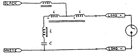
Figure 3. Power factor correction for magnetic ballast.
