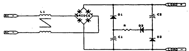
Figure 7. Passive power factor correction IV.
