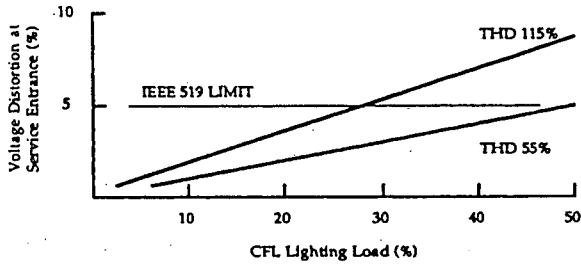
Figure 1. Voltage distortion vs. percent CFL load.
