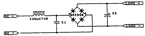
Figure 4. Passive power factor correction I.
