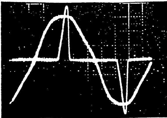
Figure 2. Typical voltage and current wave form for an IBM computer power supply unit. The sine wave is the input line voltage wave form and the spiked wave is the input current. This produces extremely high harmonic distortion and the measurement will normally measure a power factor of .4-.6. The types of losses associated with this type of distortion can be significantly greater than the losses associated with the .5 power factor.
