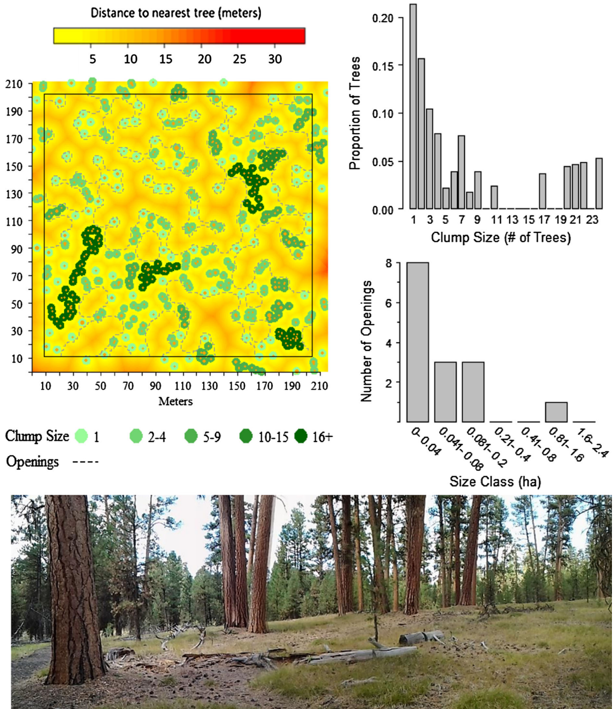
Fig. 10 Stem map ( top left panel ) and corresponding clump and opening size distributions ( right panels ) from a 4 ha plot of a reconstructed 1880 CE ponderosa pine forest on the Fremont–Winema NF, Oregon. Background color gradient shows the distance to nearest tree. A 3 m crown radius was used to project
