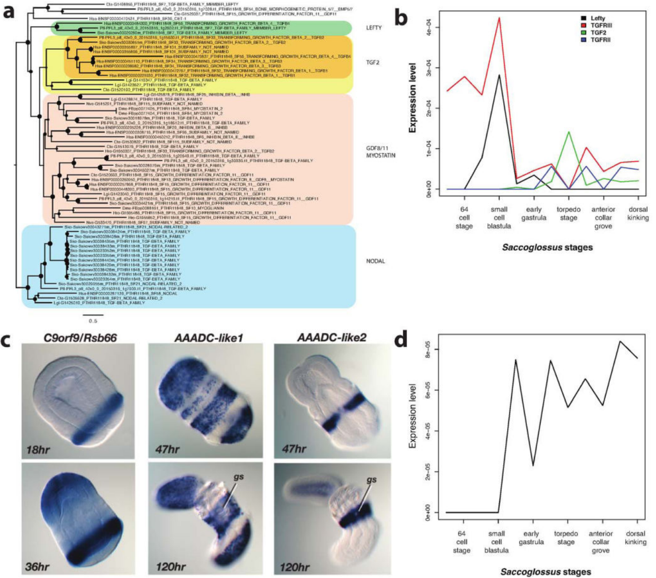
Extended Data Figure 9. Gene innovation in deuterostomes a , FastTree phylogenetic tree of the TGFβ family members Lefty, TGFβ 2, GDF8/11 and Nodal ligands (using GTR model). Bootstrap support is plotted as filled circles (size proportional to the support value) on each node. While Lefty shows deuterostome unique sequence composition, TGFβ 2 has an acceleration of sequence change at the deuterostome stem branch, compared to the GDF8/11 or Nodal groups. b , Temporal co-expression of Lefty and TGFβ receptor type III in Saccoglossus at pre-gastrulation developmental stages and of TGFβ 2 and TGFβ receptor type II at post-gastrulation stages. c , In situ hybridization demonstration of the expression in S. kowalevskii of one of the putative type I novelty genes ( c9orf9 , also known as rsb66 ) and of two of AAADC genes (aromatic amino acid
