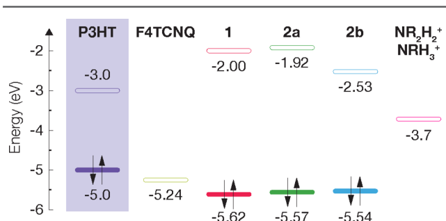
Figure 5. Energy levels of P3HT, F4TCNQ, and F4TCNQ–amine products obtained from CV and UV–vis spectroscopy. Filled bars indicate HOMO levels; unfilled bars indicate LUMO levels. See Supporting Information Section 3 for CV data.
