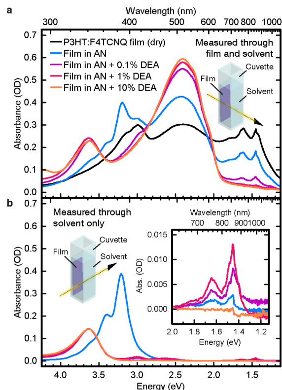
Figure 3. In situ UV-vis spectroscopy of reactive dedoping. (a) Spectra of P3HT:F4TCNQ films dry before immersion, immersed in a cuvette containing AN, and immersed in AN solutions containing varying amounts of DEA. (b) Spectra of the same samples rotated 90° to measure the solvent only. Inset shows F4TCNQ ^{\bullet-} absorption. Solution spectra were collected after 5 min of immersion; film + solution spectra were collected after 7 min of immersion.
