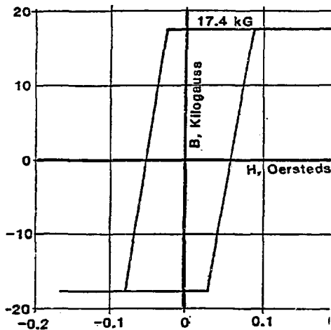
Fig. 5 Hysteresis curve of 2605 CO metallic glass.
