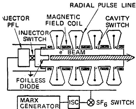
Fig. 4 Radlac: radial line geometry
