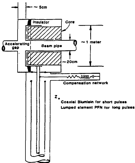
Fig. 1 Induction Acceleration Cavity and Voltage Generator
