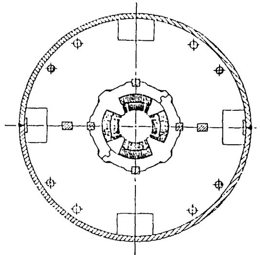
Fig. 4. Cross section of coil in iron yoke.
