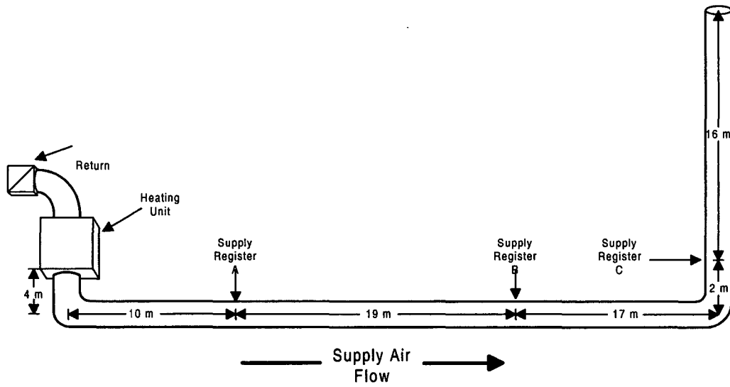
Figure 4. Registers and supply duct layout in duct System L2 (heating, long duct).
