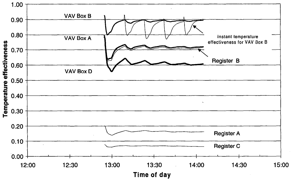
Figure 7. Short-term temperature effectiveness for VAV boxes and registers.
