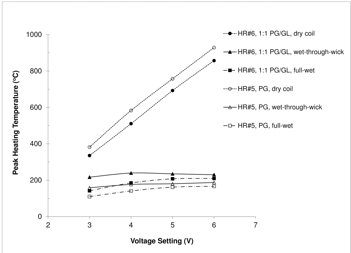
Fig 5. Peak heating temperature measured for different e-liquid fill levels and e-liquid compositions as a function of voltage setting. Note: HR = high resistance; button activation cycle = 4 s activation every 30 s; test liquid = propylene glycol (PG) or a 1:1 (wt/wt) mixture of propylene glycol and glycerol (PG/GL).
