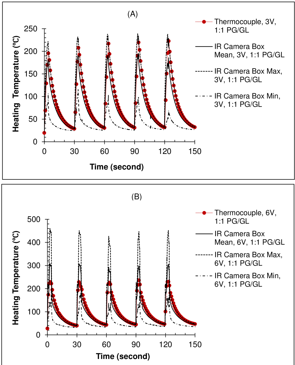
Fig 6. Comparison of thermocouple and infrared (IR) camera temperature measurements for coil HR #6 under the wet-through-wick condition: (A) 3 V; and (B) 6 V. Note: HR = high resistance; button activation cycle = 4 s activation every 30 s; test liquid = 1:1 (wt/wt) mixture of propylene glycol and glycerol (PG/GL); see Fig 1 for measurement set-up.
