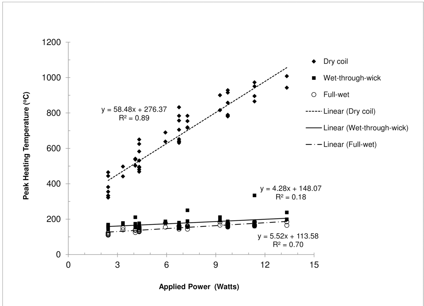
Fig 3. Peak heating temperature measured for different voltage settings, coil resistances, and e-liquid fill levels as a function of applied power. Note: button activation cycle = 4 s activation every 30 s; test liquid = propylene glycol.
