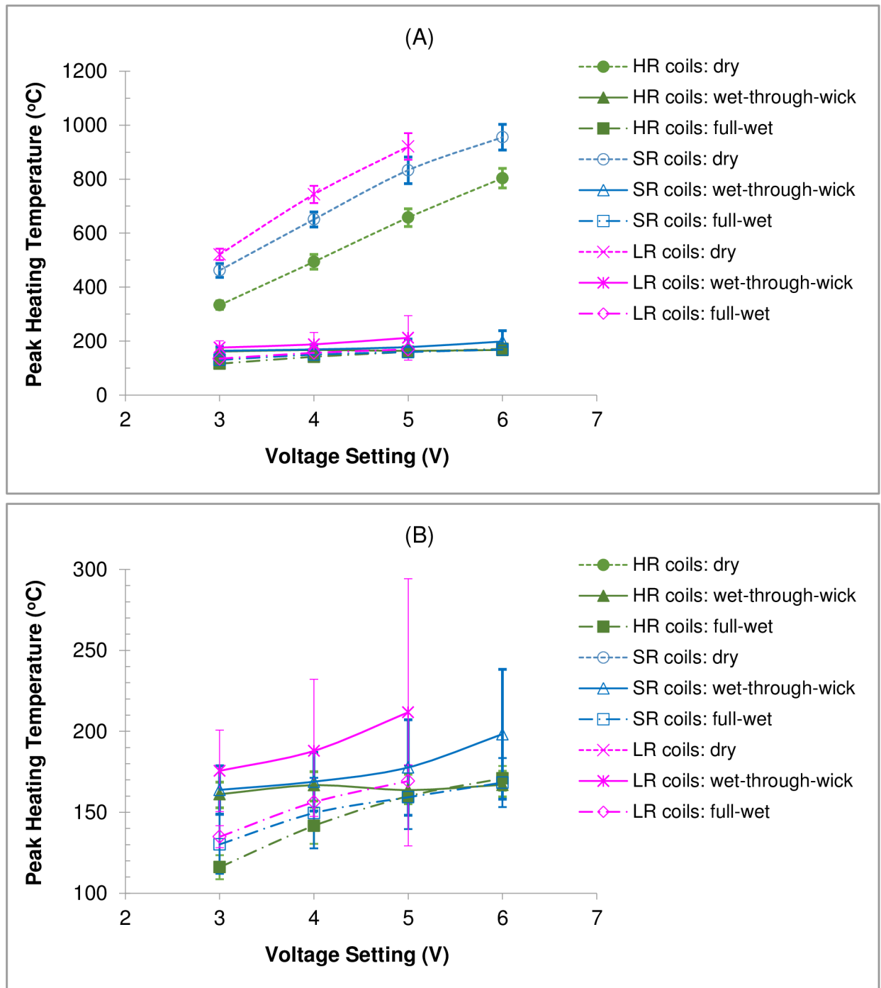
Fig 2. Peak heating temperature for different coil resistances and e-liquid fill levels as a function of voltage setting: (A) full scale; and (B) enlarged scale. Note: the average temperature \pm one standard deviation is presented for four coils tested at each resistance level; LR = low resistance, SR = standard resistance, and HR = high resistance; button activation cycle = 4 s activation every 30 s; test liquid = propylene glycol.
