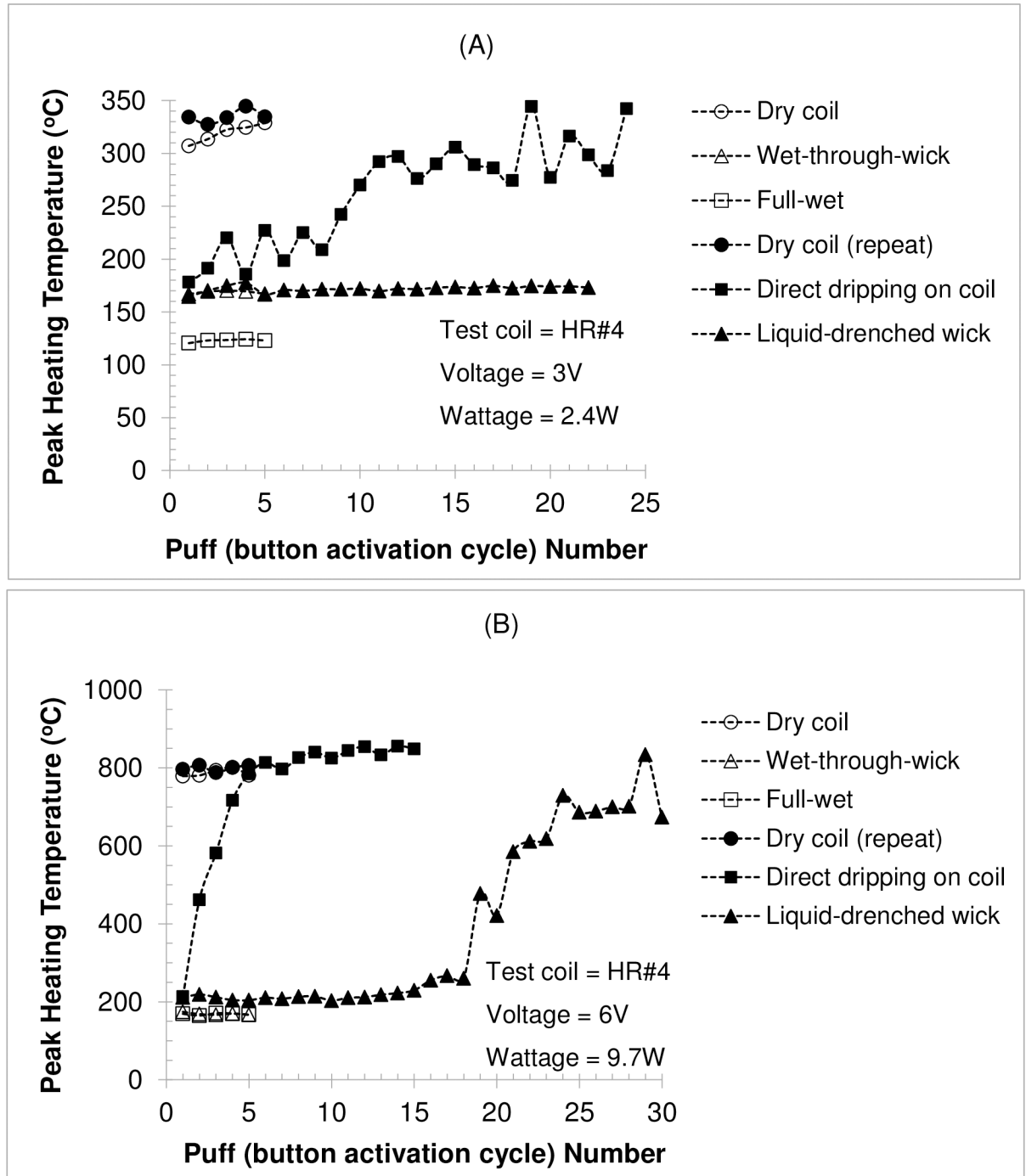
Fig 4. Peak heating temperature measured for coil HR #4 under various coil conditions: (A) 3 V; and (B) 6 V. Note: HR = high resistance; button activation cycle = 4 s activation every 30 s; test liquid = propylene glycol.
