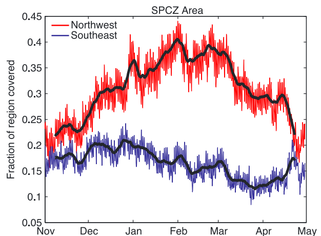
Figure 6. Mean SPCZ area over 1980–2011 seasons for the northwest ( 0^{\circ} – 15^{\circ}\text{S} , 130^{\circ}\text{E} – 170^{\circ}\text{W} ) and southeast ( 15^{\circ}\text{S} – 30^{\circ}\text{S} , 170^{\circ}\text{W} – 110^{\circ}\text{W} ) regions in units of fraction of region covered. Red and blue curves show the 3-hourly areas while black curves show the 7 day running means.
