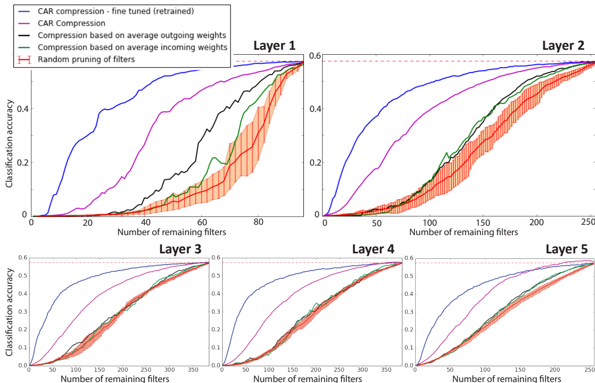
Figure 2.3: Performance of CAR compression for AlexNet. Each panel shows the classification accuracy of the AlexNet when an individual convolutional layer is compressed. In each panel, the classification accuracy of uncompressed network is shown with a dashed red line. The purple curve shows the classification accuracy of our proposed CAR compression algorithm for various compression ratios. The accuracy for the fine tuned (retrained) CAR compression is shown in blue. The black and green curves shows the accuracy for compressed network based on outgoing and incoming weights, respectively. The red curve shows the accuracy when filters are pruned uniformly at random. The error bar is reported over 10 repeats of this random pruning process.
