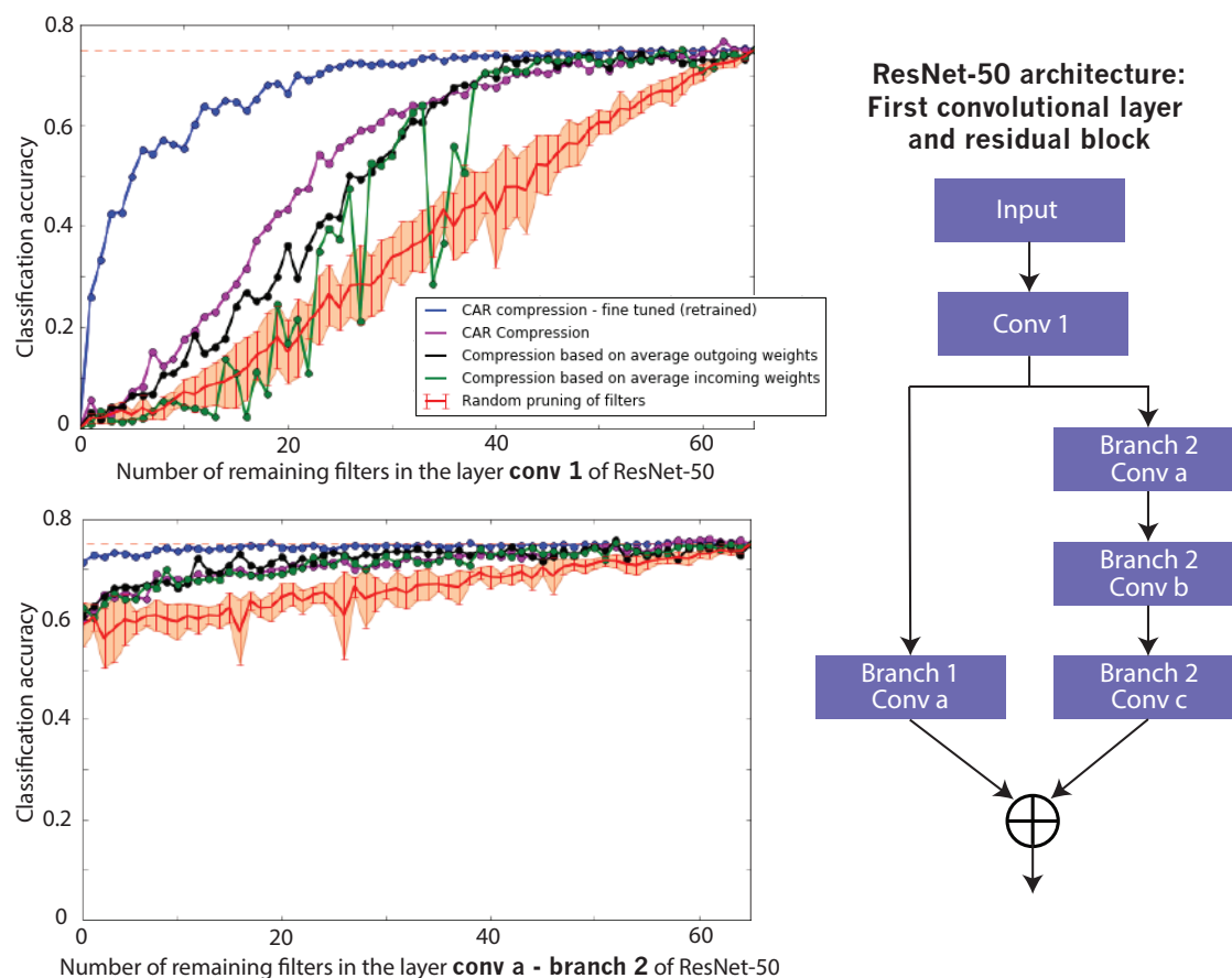
Figure 2.4: Performance of CAR compression for ResNet-50. The top left figure shows the classification accuracy of the ResNet-50 when the first convolutional layer is compressed. The bottom left figure shows the classification accuracy when filters in the first residual module layers are pruned (with the first layer untouched). The classification accuracy of uncompressed network is shown with a dashed red line. The purple curve shows the classification accuracy of our proposed CAR compression algorithm for various compression ratios. The accuracy for the fine tuned (retrained) CAR compression is shown in blue. The black and green curves shows the accuracy for compressed network based on outgoing and incoming weights, respectively. The red curve shows the accuracy when filters are pruned uniformly at random. The error bar is reported over 10 repeats of this random pruning process. The right panel shows the architecture of first layers in ResNet-50.
