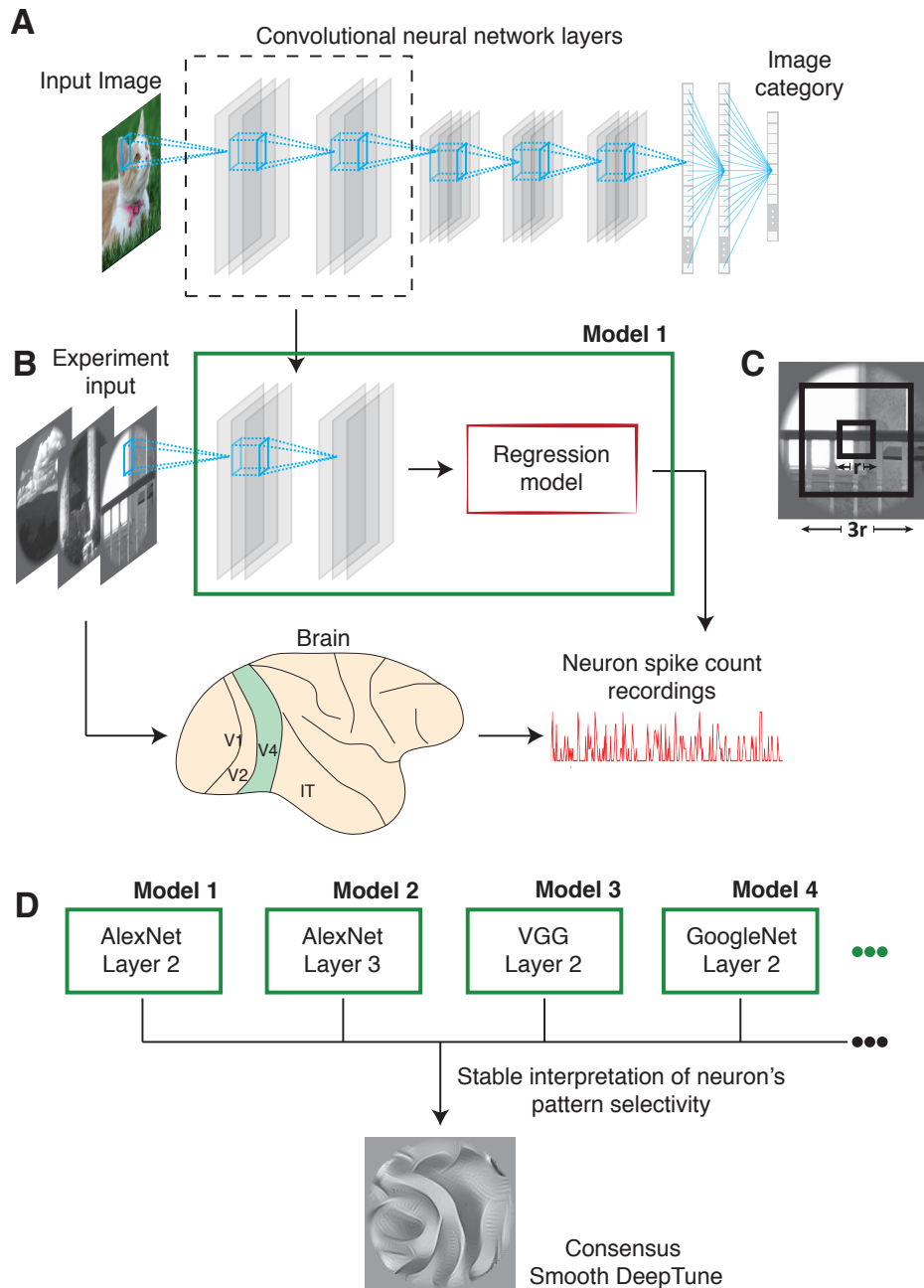
Figure 3.1: Transfer learning of pre-trained convolutional neural networks to predict spike rates of neurons in the area V4 and the stability-driven interpretation. A. A convolutional neural network trained to perform 1000-class image classification task on ImageNet dataset which contains more than 1.2 million natural images. In this chapter, three well-known CNN structures have been used: AlexNet, VGG and GoogleNet. B. Weights from early layers of the trained CNN are fixed and transferred
