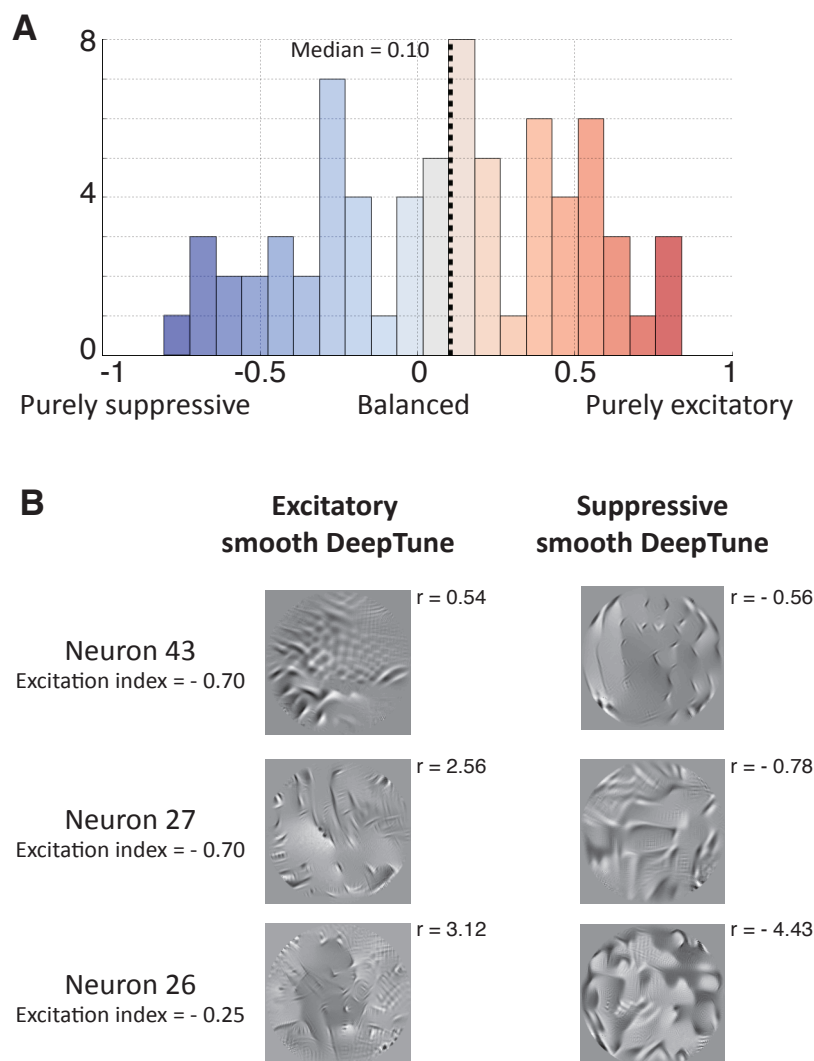
Figure 3.7: Neurons in cortical area V4 exhibit suppressive tuning. A. Histogram of excitation index for 71 V4 neurons. 41% of the neurons show strong suppressive tuning. The median of excitation index for V4 neurons is 0.10. B. The excitatory and inhibitory smooth DeepTune images for three neurons identified as suppressive by the STRF model and excitation index. The neuron excitation index and response of the model to each smooth DeepTune image is illustrated in the same panel. The neurons with suppressive tuning tends to have a clearer suppressive DeepTune visualization than those without.
