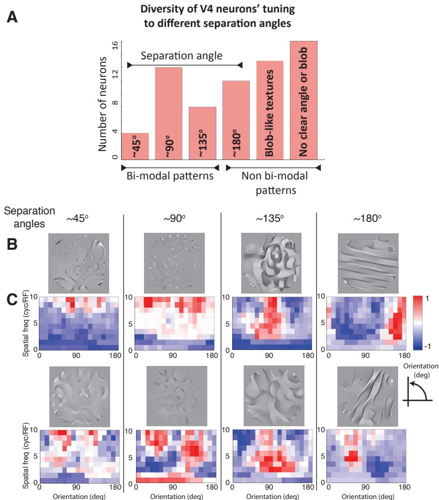
Figure 3.6: Categorization of V4 neurons based on their separation angles. A. Neurons are manually categorized into six groups. The first four groups contains neurons tuned to patterns with separation angles of 45^\circ , 90^\circ , 135^\circ , and 180^\circ . These patterns are either contours or textures. About 20% out of 71 neurons are tuned to patterns with separation angles of 90^\circ . Another 20% of the neurons are selective to blob-like textures which does not correspond to any particular angle. The rest of neurons are not selective to any clear angle or blob-like patterns. B. The consensus smooth DeepTune image for two example neurons in each of the first four categories and C. the corresponding spectral receptive field (SRF) (David et al [12]) visualization. The orientation tuning obtained via SRFs and consensus DeepTune images are consistent. while SRF predicts a neuron has tuning for a particular angle through Fourier analysis, the consensus DeepTune images offer concrete visualization of these tunings. For example, for the bottom left neuron, both our method and SRF show an orientation tunings of about 70^\circ and 120^\circ .
