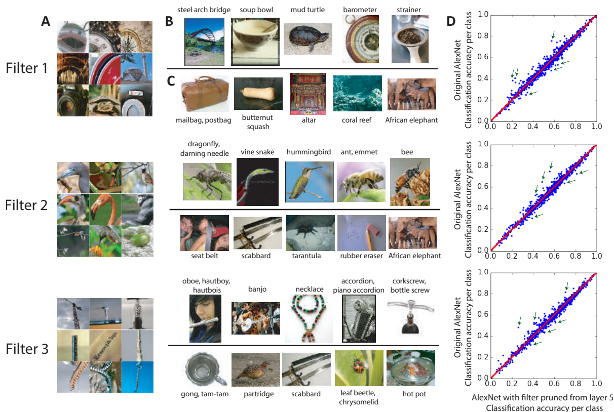
Figure 2.7: The interpretation based on CAR^c is consistent with the visualized pattern selectivity of each filter in layer 5 of AlexNet. Panel A shows The top 9 image patches that activate each filter [74]. Panel B and C show the top and bottom 5 classes with highest and lowest CAR^c , respectively. Besides the class label, one sample image from that class is also visualized. Panel D shows the scatter plot of classification accuracy for each of the 1000 classes in ImageNet. Three of the top and bottom classes with highest and lowest CAR^c are pointed out with green arrows. Each row corresponds to one filter in layer 5 of AlexNet.
