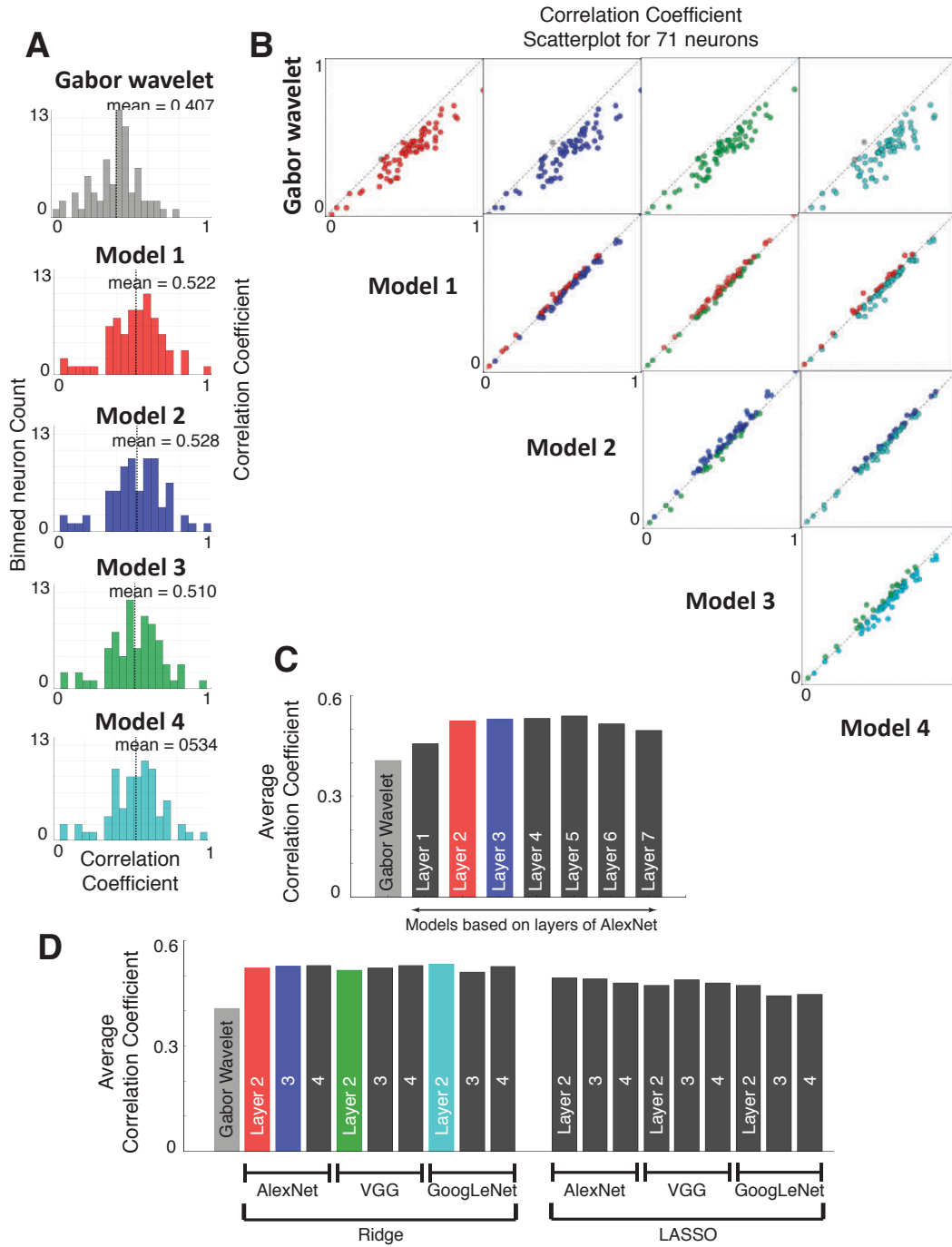
Figure 3.2: CNN-based models have better prediction performance compared to Gabor wavelet model. Noise-corrected correlation coefficient [60] is used as prediction performance measure in this figure. A. Histogram of correlation coefficients over population of V4 neurons for four models are shown in the first column. B. Scatter plots
