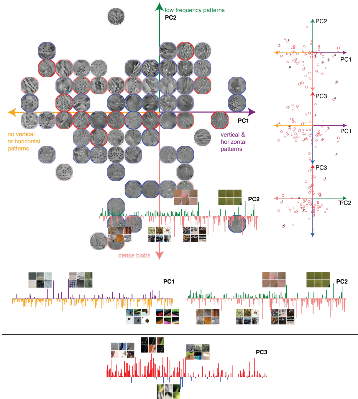
Figure 3.G.1: Principle components analysis of V4 neuron's population. A. 71 V4 neurons according to their values in the first two principal components. To compute the principle components, we perform \ell^2 pooling of coefficient values across space and time delays to yield a single impact value for each of the filters in layer N2 of AlexNet. This
