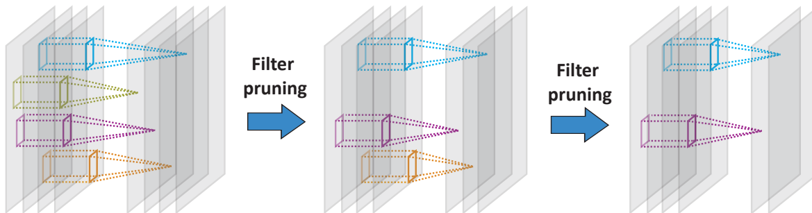
Figure 2.1: Greedy compression of CNNs based on pruning filters.
