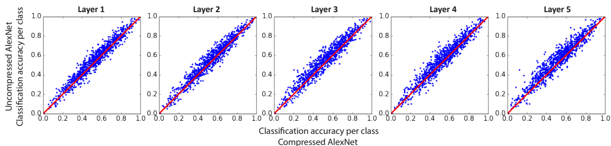
Figure 2.6: Comparison of classification accuracy between compressed and uncompressed networks for each class of image in AlexNet. Each panel corresponds to compression in one layer. Each point in plots corresponds to one of the 1000 categories of images in ImageNet test set.
