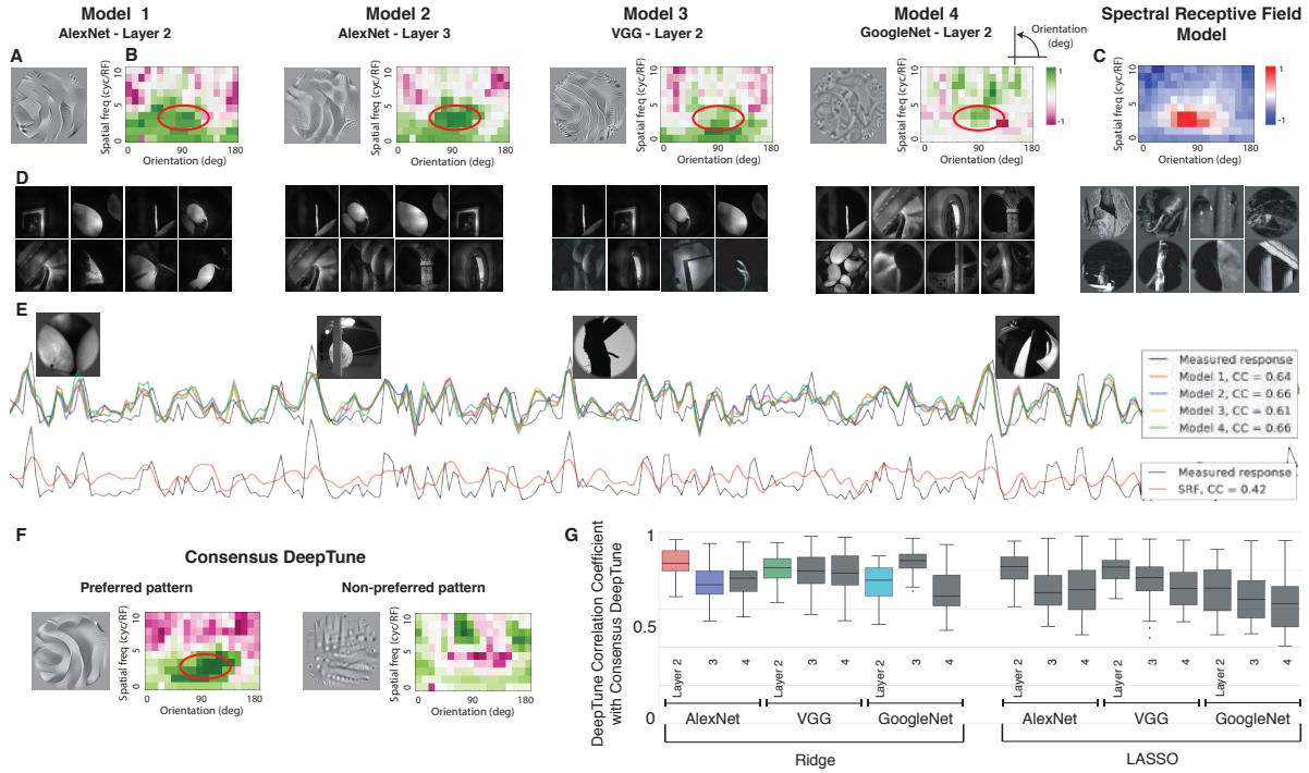
Figure 3.3: For single neuron, smooth DeepTune images are stable across models. A. Smooth DeepTune images based on four main models are shown for neuron 1. Note that these images share a visually stable curvature pattern with edges forming an approximately 90 degree angle (Also visible in the rest of our 14 models - see Appendix, Figs. S8 and S9 ). B. Power spectral density (PSD) of the smooth DeepTune images in polar coordinates. All four DeepTune images share a strong and stable frequency component in the range of 45 to 135 degrees with spatial frequency of 2 to 5 cycle per receptive field (the green color). C. Visualization of spectral receptive field (SRF) [12] model for neuron 1. The SRF visualization emphasizes in red the frequency components of the stimulus image selected by its regression model and therefore we use a different color-map (red-blue) than that for the DeepTune PSD image (green-pink). The pattern selectivity according to SRF is consistent with the stable parts of smooth DeepTune (highlighted in red circle). D. Images from training set with the highest responses for neuron 1. Similar curvature patterns to the smooth DeepTune visualization are visible in these images. E. The measured and predicted spike rates in the test set from the four main models as well as the SRF model for neuron 1. Images from the test set with the highest responses are visualized on top of the corresponding spike rate. Similar curvature patterns are visible in these images. Correlation coefficient between the measured and predicted spike rates is shown in the right panel. All of the four models outperform the SRF model. F. The consensus smooth DeepTune image for neuron A. Both preferred and non-preferred
