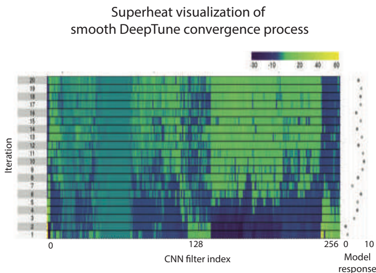
Figure 3.D.1: The smooth DeepTune image optimization process. We use SuperHeat visualization package to plot the heatmap of the CNN feature activation map throughout the optimization process.
