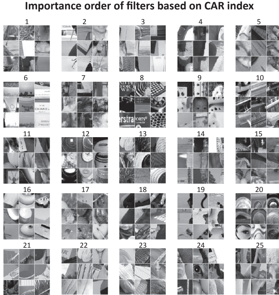
Figure 4.3: Visualization of filters in the second layer of AlexNet with the highest CAR index. To visualize a convolutional filter from a CNN, we show the 9 top image patches from the ImageNet training set that has the highest filter responses. The filters are ordered based on their CAR importance index.
