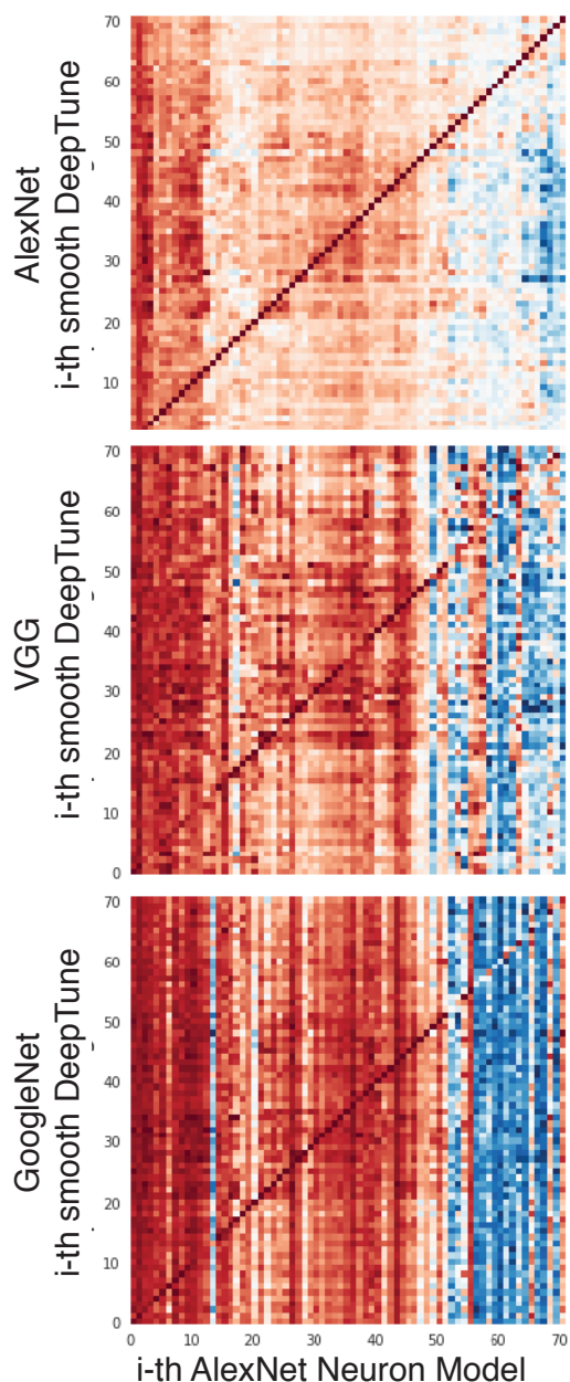
Figure 3.D.4: Stability of model responses to smooth DeepTune images generated from AlexNet, Vgg, and GoogleNet based models. Smooth DeepTune images from layer 2 of AlexNet, VGG and GoogleNet are generated for each neuron. These images are fed into our prediction model based layer 2 feature of AlexNet. All three heatmaps contain clear diagonal pattern, showing the smooth DeepTune images are stable across models. This observation, quantitatively confirms the visually observed stability of smooth DeepTune images.
