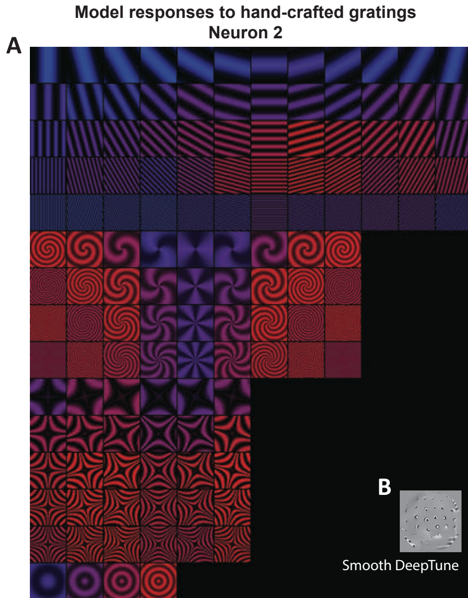
Figure 3.H.2: Neuron 2 model responses to polar, hyperbolic, and Cartesian gratings are consistent with smooth DeepTune patterns. A. Responses of neuron 2 model to polar, hyperbolic, and Cartesian gratings. The gratings in red and blue correspond to excitatory and inhibitory stimulus, respectively. B. Smooth DeepTune of neuron 2
