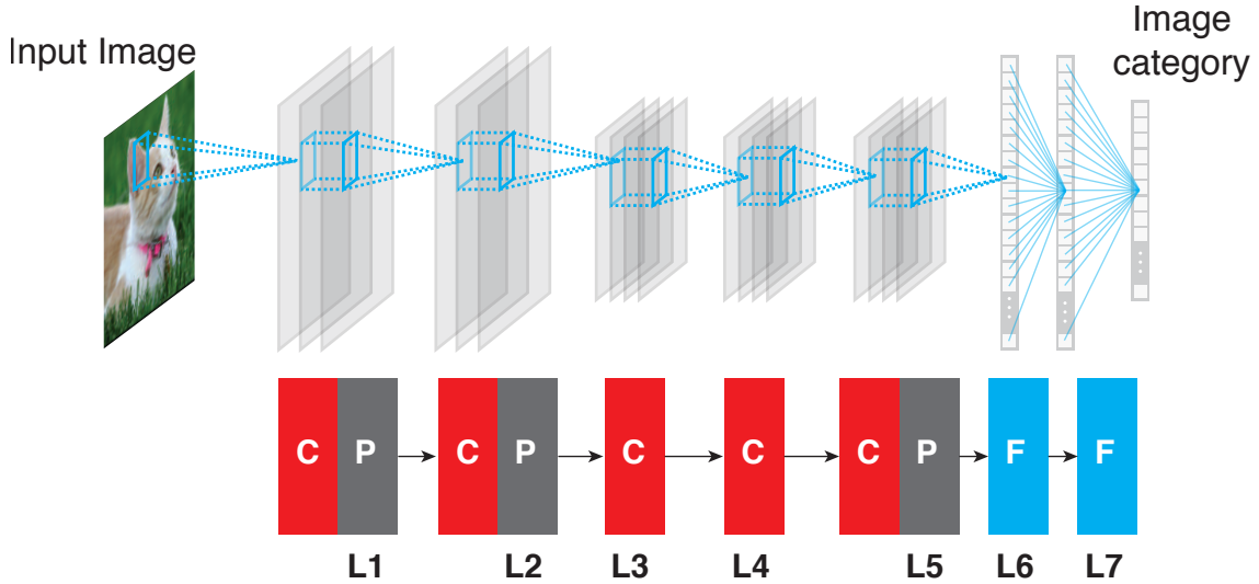
Figure 3.B.1: Architecture of the AlexNet model [33] . Red box indicates convolutional layer, gray box indicates pooling layer and blue box indicates fully connected layer.
