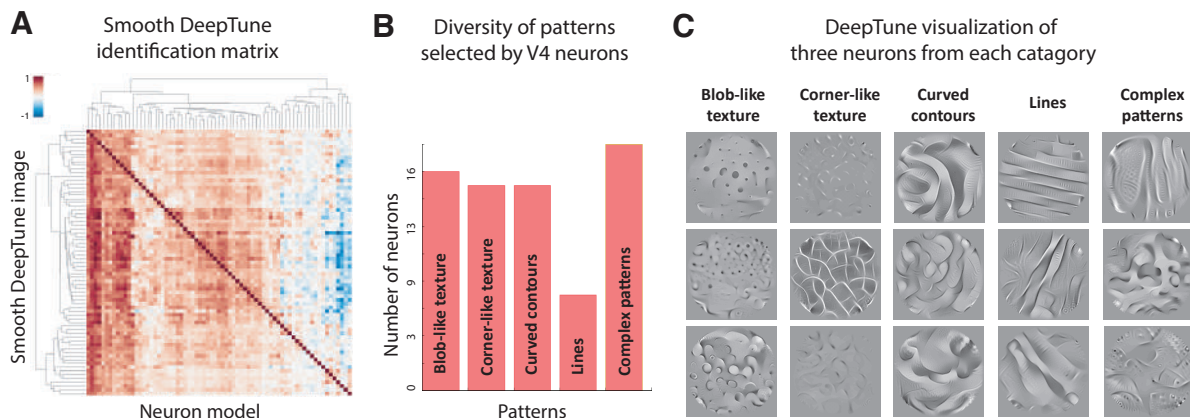
Figure 3.5: Diversity of tuning among V4 neurons. A. Responses of models for 71 neurons to all of the 71 consensus smooth DeepTune images are shown in the identification matrix. All models are based on AlexNet layer 2 with l_2 regularization in regression. A clear diagonal line is formed which demonstrates that for each neuron, the consensus DeepTune image has the highest response to its own model compared to that of other neurons' models. B. Neurons are manually categorized into five categories based on their smooth DeepTune images. More than 40% of the neurons are selective to texture patterns, half of which prefer blob-like textures and the other half prefer corner-like textures. About 30% of the neurons exhibit contour patterns, both curvature and straight lines. Neurons selective to curvatures are twice as the ones selective to straight lines. The rest of the neurons have selectivity to visually complex patterns. C. Examples of consensus DeepTune images for three neurons from each of the five categories.
