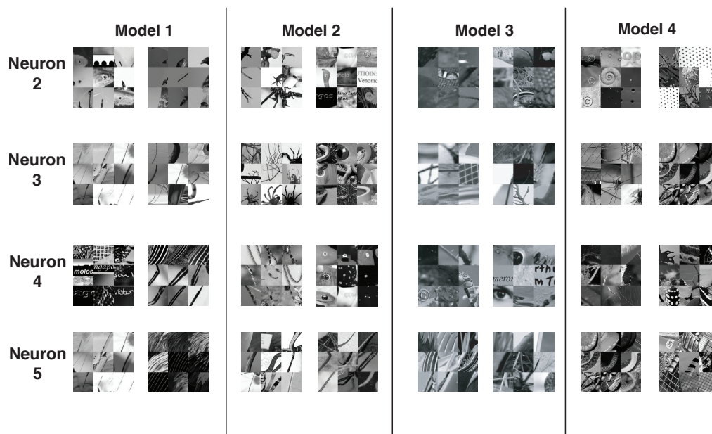
Figure 3.D.5: Stability of top selected CNN features selected by each neuron across four main models. Each box visualizes a filter representing the feature in the CNN. To visualize the filter, we feed a million random natural images (from AlexNet dataset) to the network and show the top 9 image patches that activate the filter.
