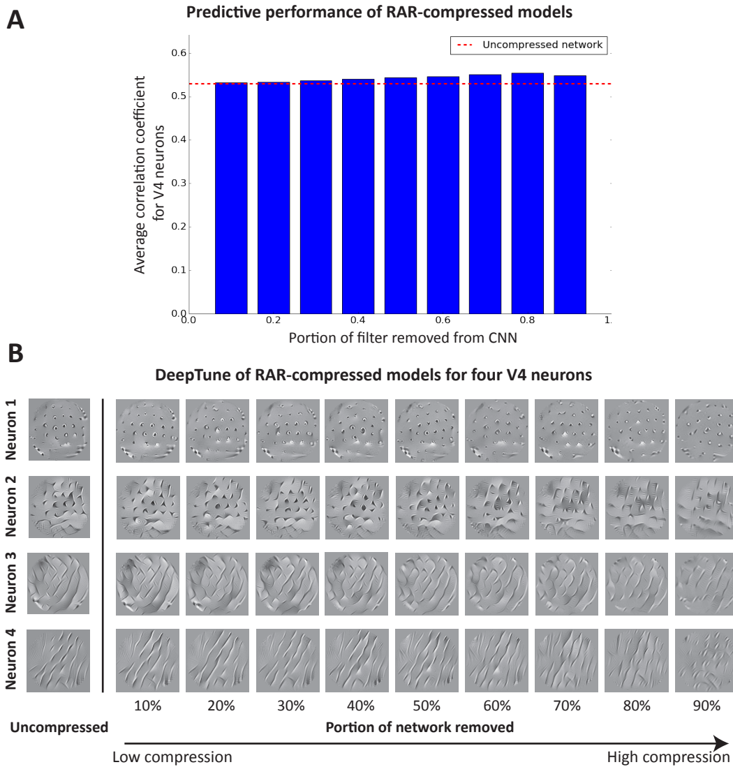
Figure 4.4: Performance of RAR-compressed networks in predicting spike rates of neurons in visual area V4. A. Average correlation coefficient over 71 neurons for RAR compressed networks with various compression rates. The model is based on AlexNet layer 2 with Ridge regression. The red dashed line shows the average correlation coefficient for the uncompressed network. B. DeepTune visualization of pattern selectivity for RAR-compressed models. The DeepTune images for four neurons and 9 different compression rate are shown. The compressed models have stable patterns compared to uncompressed models up to 90% compression rate. For Neuron 3, the pattern is enhanced in higher compression rates.
