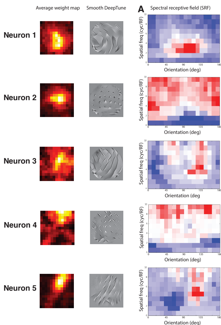
Figure 3.F.1: Consistency of the average weight map and smooth DeepTune images with spectral receptive field (SRF) [12]. Details of the SRF model are discussed in the main text.
