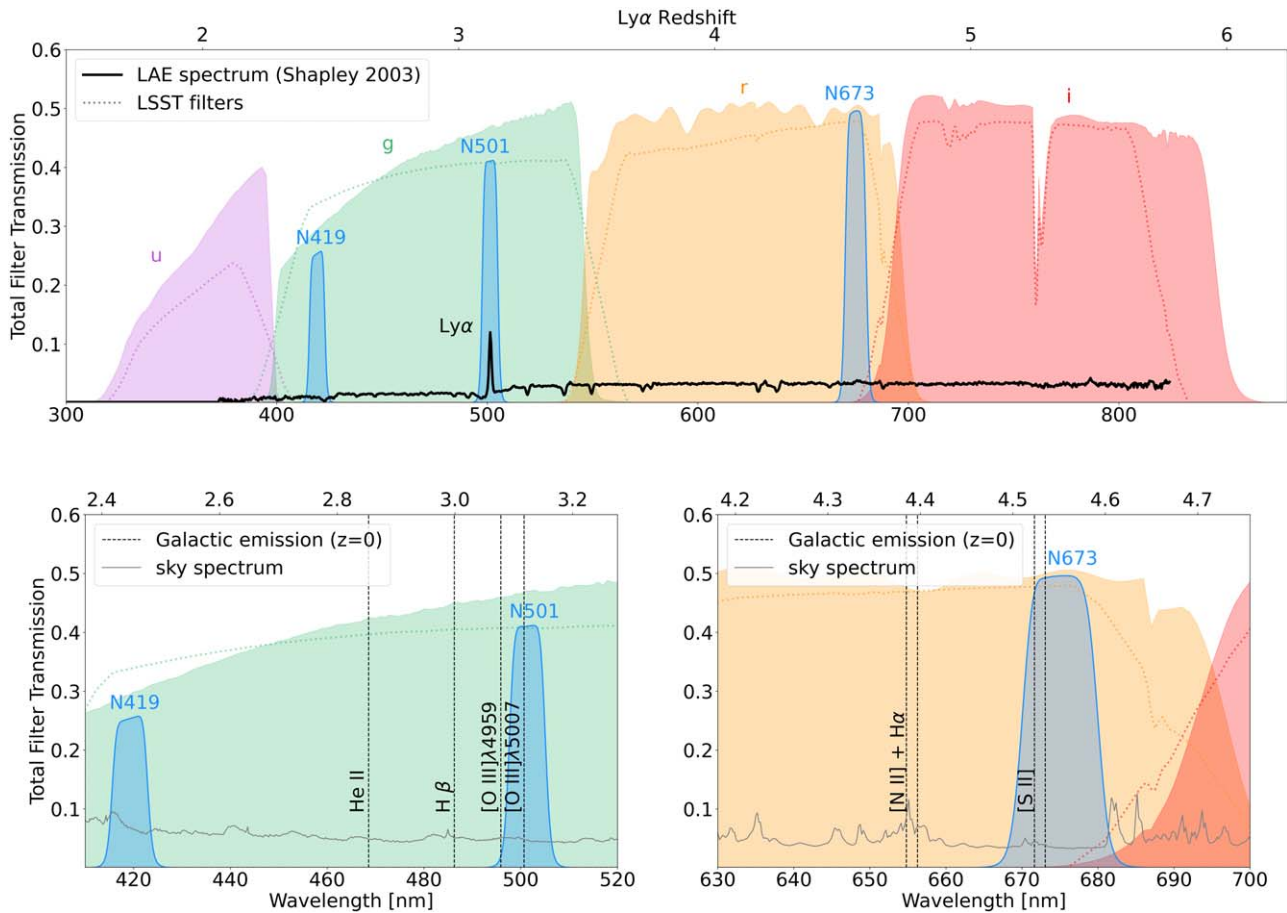
Figure 1. Top: ODIN narrowband filters made for DECam (blue shaded regions; from left to right, N419 , N501 , and N673 , respectively) together with the transmission curves for the broadband filters from Subaru HSC ( gri ) and CFHT/MegaCam ( u ). Future LSST passbands for the same broad bands are shown as dotted lines. These imaging data are combined to isolate redshifted Ly \alpha emission falling into the narrowband filters as illustrated by the template LAE spectrum (black) at z = 3.1 . The Ly \alpha redshift range is shown at the top. Bottom: zoom-in views of the three ODIN filters. Overlaid are strong Galactic emission lines (vertical dotted lines) and the sky spectrum (gray curves). N501 and N673 sample the [O III] \lambda 5007 and [S II] emission from Galactic sources and nearby galaxies.
