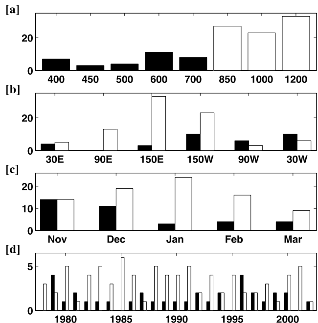
Figure 2. Histogram of identified strong PWB events in the NH stratosphere by (a) isentropic surface, (b) longitude, (c) month, and (d) year. Upper-level PWB events, identified on and above 850 K, are indicated in white. Lower-level PWB events, identified on and below 700 K, are indicated in black.
