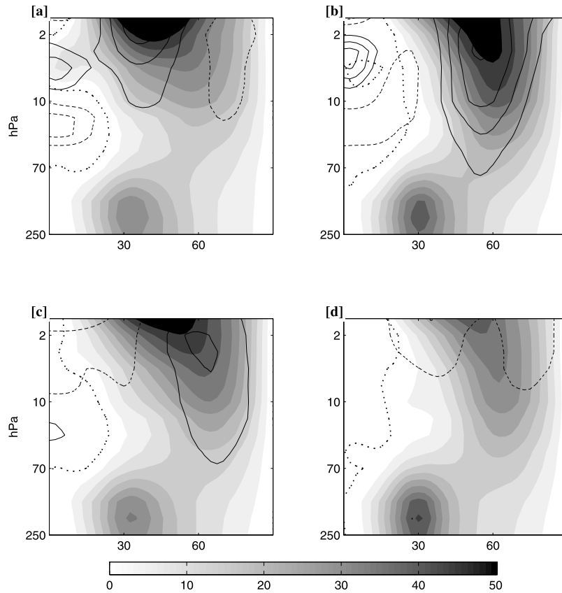
Figure 3. Composite zonal-mean zonal velocity \bar{u} averaged over early winters (1 Nov–31 Dec.) with (a) multiple lower breaking events, and (b) multiple upper breaking events. The composite \bar{u} averaged over mid-winters (21 Dec–10 Feb.) following early winters with (c) multiple lower and (d) multiple upper breaking events. Shading shows \bar{u} values, the dotted contour indicates the zero wind line, and positive (negative) anomalies are shown by solid (dashed) contours with a contour interval of 3 \text{ ms}^{-1} .
