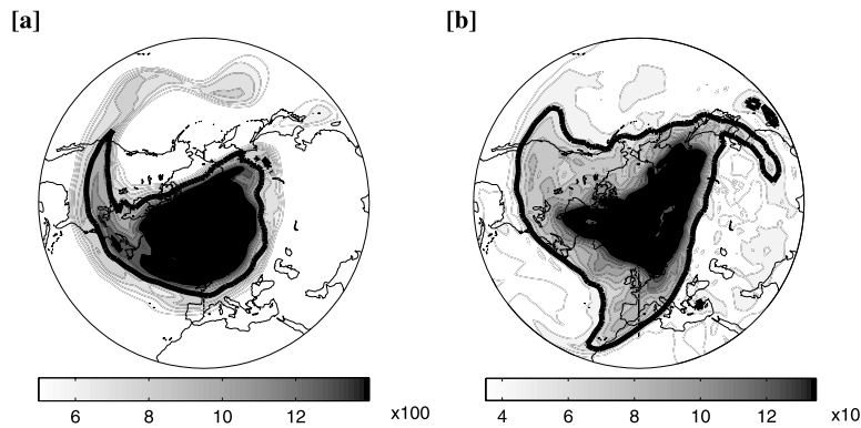
Figure 1. Examples of breaking in the (a) upper stratosphere on the 1000 K isentropic surface occurring on 16 December 1982, and (b) lower stratosphere on the 600 K isentropic surface occurring on 6 January 1979. Potential vorticity (PV) is shaded and shown in PVU, and the bold contour represents the vortex edge ( PV_{\theta} ) as described in the text.
