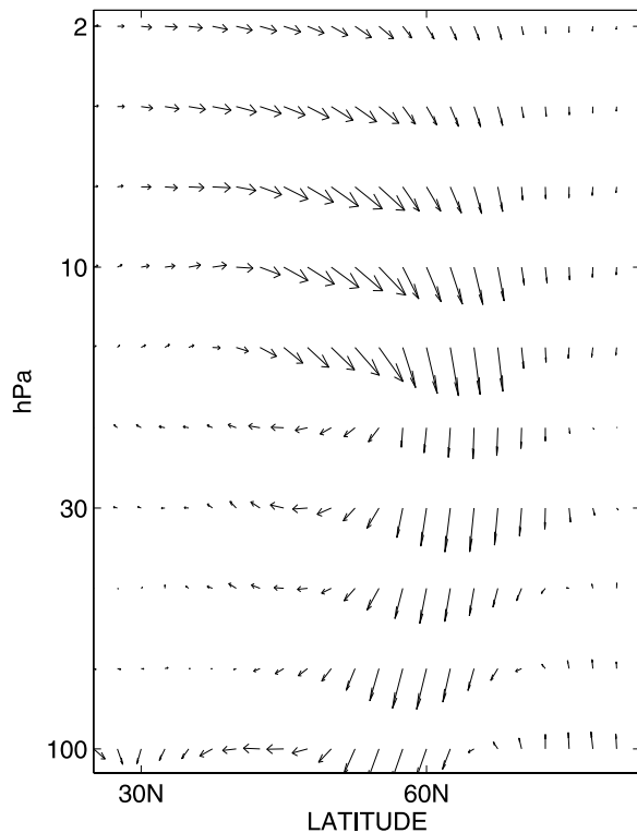
Figure 4. The composite EP flux difference averaged over 1 Nov–31 Dec. for periods with multiple lower breaking events minus periods with multiple upper breaking events, and multiple lower breaking events. Maximum vector shown is of magnitude 1.2 \times 10^5 \text{ kg s}^{-2} . The EP vectors are scaled by multiplying the horizontal component by 85.
