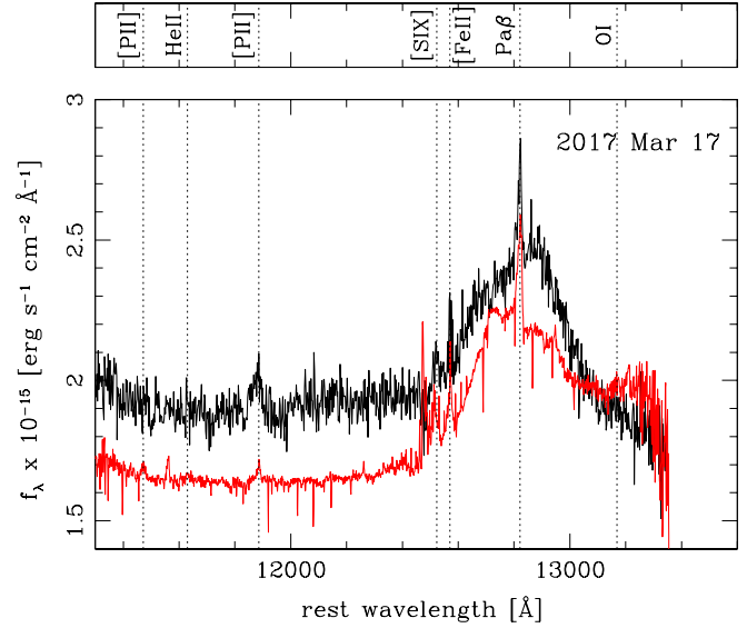
Figure 3. IRTF SpeX near-IR spectrum from 2017 March 17 (black) compared to the NIFS J band spectrum obtained by summing the flux in a 0.3'' \times 1.2'' aperture centered on the nucleus and oriented at the same position angle as the IRTF spectral aperture (red). The main emission lines are identified and labeled.
