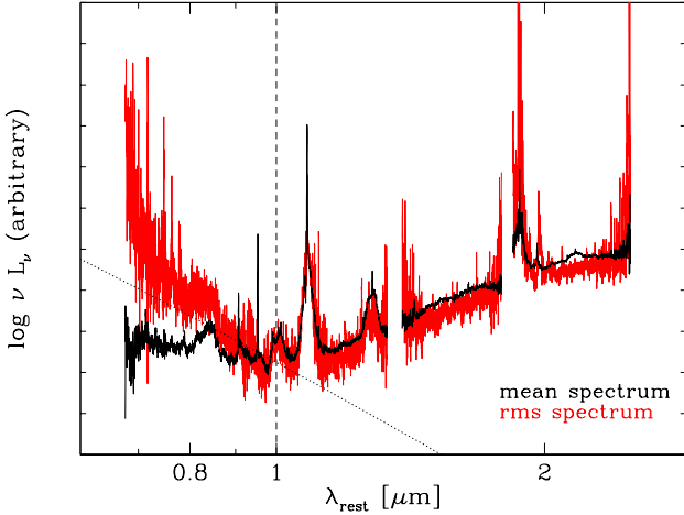
Figure 7. The mean (black) and variable (rms) spectrum (red) for our campaign normalised at rest-frame 1 \mu\text{m} (vertical dashed line). The spectrum of a standard accretion disc (black dotted line) approximates well the wavelength range of 0.7\text{--}1 \mu\text{m} for the variable component, which is observed to be much bluer than the mean spectrum (similar to the result from the 2014 HST reverberation campaign; see Fig. 6). The spectral shape at wavelengths \gtrsim 1 \mu\text{m} is similar in the mean and rms spectrum.
