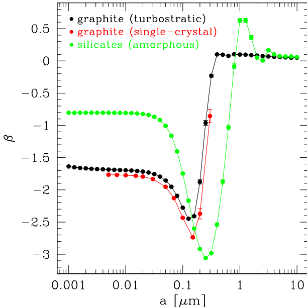
Figure 8. Power-law slope \beta versus the grain size for turbostratic graphite (black), single-crystal graphite (red) and amorphous silicates (green). We have fitted the relationship Q_\lambda(a) \propto \lambda^\beta in the wavelength region of \lambda = 1 - 3 \mu\text{m} the data calculated by Draine (2016) for graphite and by Draine & Hensley (2017) for silicates.
