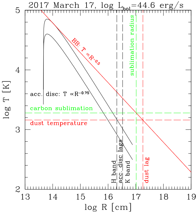
Figure 13. The temperature-radius relationships for the accretion disc (black curves) and hot dust (red curve) for the observation from 2017 March 17. The red horizontal and vertical dashed lines indicate the observed dust temperature ( T \sim 1450 K) and reverberation radius ( R_{d,rev} \sim 70 light-days), respectively. The green horizontal and vertical dashed lines indicate the expected carbon sublimation temperature ( T \sim 1900 K) and radius ( R_{d,sub} \sim 40 light-days), respectively. The black vertical dashed lines indicate the peak lag times in the H and K bands assuming for the response function the temperature-radius relationship of a standard accretion disc ( \sim 7 and 12 light-days, respectively).
