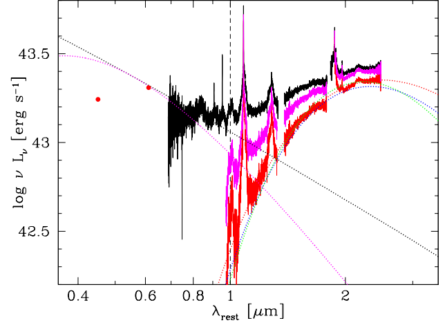
Figure 5. IRTF SpeX near-IR spectrum from 2017 March 17 shown as luminosity versus rest-frame wavelength, together with the g' and r' nuclear fluxes from the quasi-simultaneous GROND photometry (red circles). We have decomposed the continuum into an accretion disc spectrum (with a large outer radius of r_{\text{out}} = 10^4 r_g ), which approximates the wavelength range of 0.7–1 \mu\text{m} (black dotted curve) and still dominates at 1 \mu\text{m} (vertical dashed line), and a hot dust component at wavelengths > 1 \mu\text{m} (red spectrum). We have fitted the hot dust continuum with a blackbody spectrum (red dotted curve) and modified blackbody spectra for carbon and for silicate dust (green and blue dotted curves, respectively). If the accretion disc cuts off at the self-gravity radius ( r_{\text{out}} \sim 500 r_g ) or a ‘constant red component’ with a blackbody spectrum of temperature T \sim 10^4 K is assumed to dominate the emission at wavelengths \lesssim 1 \mu\text{m} (magenta dotted curve), the hot dust spectrum is broader (magenta spectrum).
