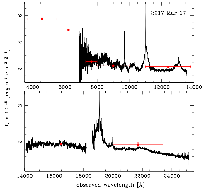
Figure 4. IRTF SpeX near-IR spectrum from 2017 March 17 (black), overlaid with the optical and near-IR nuclear fluxes from the GROND photometry of 2017 March 18 (red filled circles).
