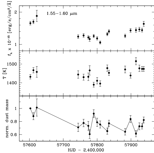
Figure 11. Temporal behaviour of the dust flux in the H band (top panel), dust temperature (for the blackbody case; middle panel) and normalised dust mass (relative to the start of the campaign and connected in time for clarity; bottom panel). We plot 1\sigma errors.
