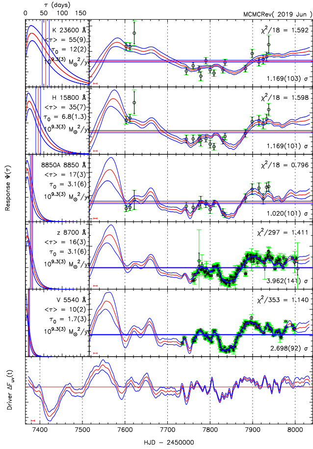
Figure 10. MCMCRev results assuming the response function of a standard accretion disc seen face-on. Symbols are as in Fig. 9. The results are summarised in Table 6.
