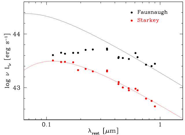
Figure 6. Photometric data from the 2014 HST reverberation campaign on NGC 5548. The mean observed AGN spectrum presented by Fausnaugh et al. (2016) (black filled circles), corrected for host galaxy starlight and line emission, is much redder than the prediction from a standard accretion disc with an accretion rate of \sim 0.1 M_{\odot} per year (black dotted line). However, the mean accretion disc spectrum inferred by Starkey et al. (2017) from fits to the observed light-curves (red filled circles) can be well approximated with a standard accretion disc, if a relatively low accretion rate of \sim 0.01 M_{\odot} per year is assumed (red dotted line).
