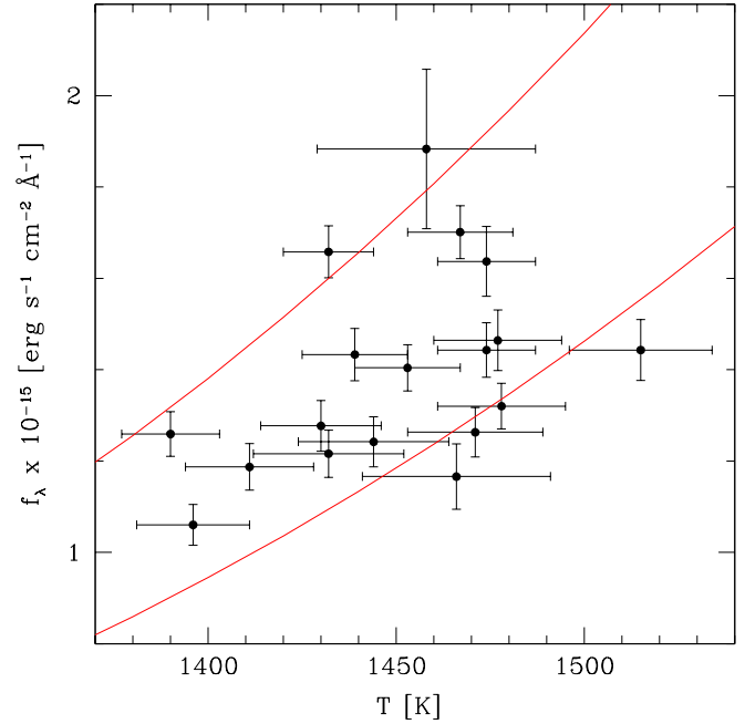
Figure 12. Flux in the wavelength region of 1.55 - 1.60 \mu\text{m} versus the temperature (for the blackbody case). We plot 1\sigma errors. The red curves show the expected relationship if the flux increase is solely due to a temperature increase. The spread in dust mass necessary to explain the flux difference between the two red curves is a factor of \sim 1.5 .
