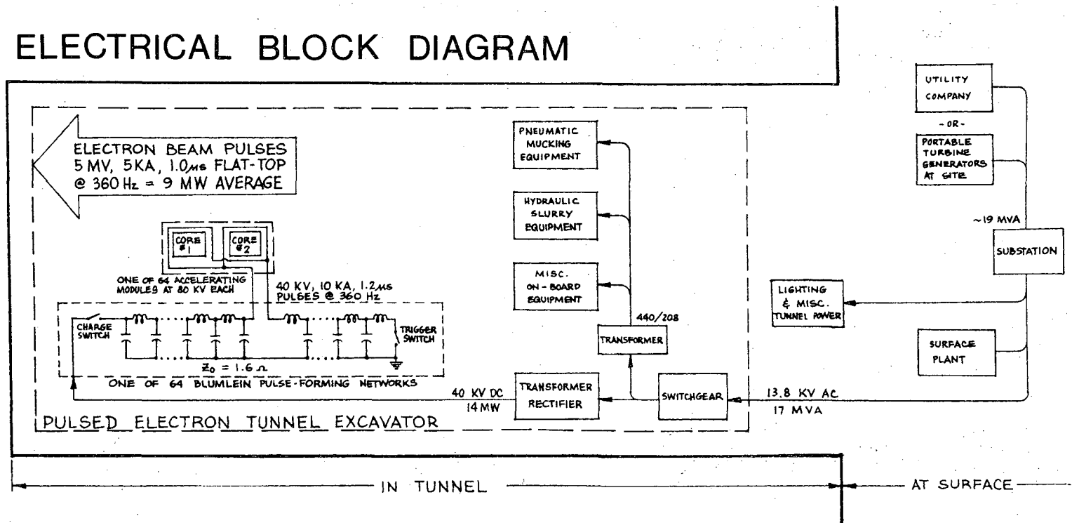
Fig. 3 - Electrical Block Diagram
