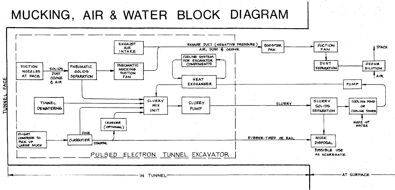
Fig. 6 - Mucking, air and water block diagram.
