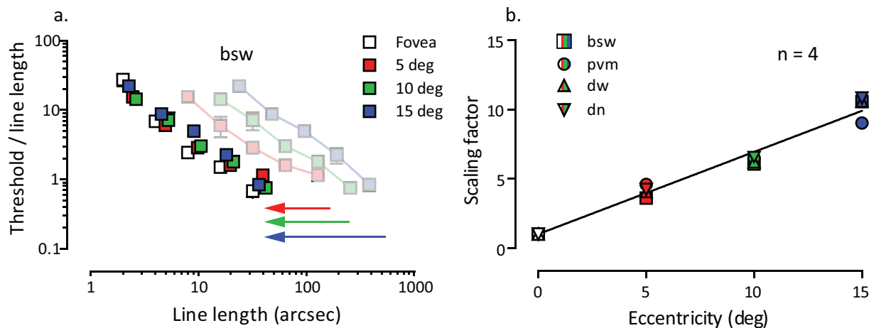
Figure 3 | Spatially scaling stimuli equates peripheral to foveal Vernier alignment thresholds. Weber fractions for the fovea and 3 eccentric locations are plotted (data shown in lower contrast) as a function of line length for a representative subject. (a) A scaling factor that minimised the mean squared error between the eccentric and foveal data (see high contrast data points) was calculated. (b) A linear regression line fitted through the data estimates the scaling factor required to increase the size of the eccentric stimuli such that performance is matched to that at the fovea. dw and dn are data reproduced from Whitaker et al. , (1992) 11 .
