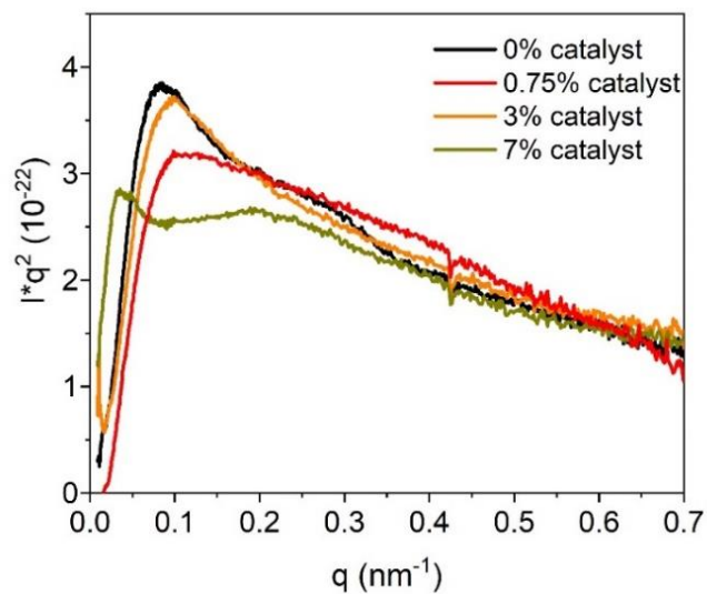
Figure S3.9. RSoXs profiles extracted at an x-ray energy of 284.2 eV and normalized by the film thickness.
