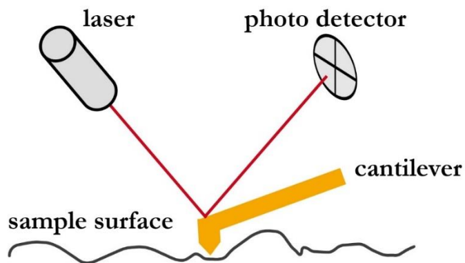
Figure 2.1. Schematic of an AFM setup in contact mode.
