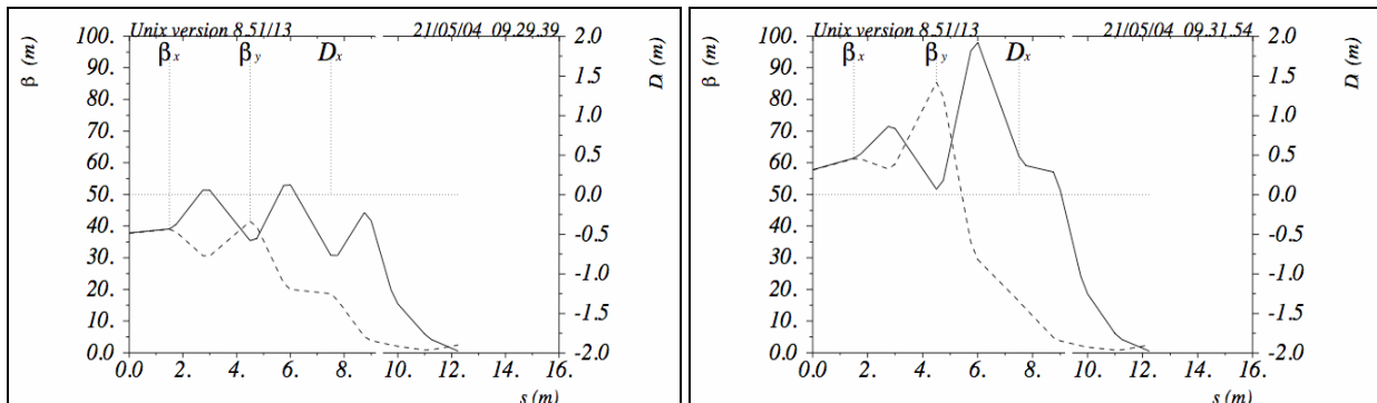
Figure 4. Beta functions for the ‘round’ beam (left) and ‘flat’ beam (right) in the ‘matching’ section.
