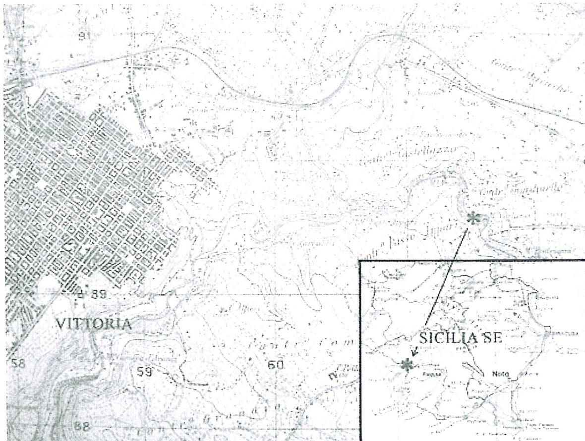
Fig. 1 - Geographical location (*) of the Cartiera Mulino section.
