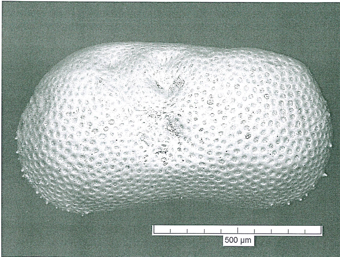
Fig. 5 - Ilyocypris gibba (Ramdohr, 1808): left valve, external view.
