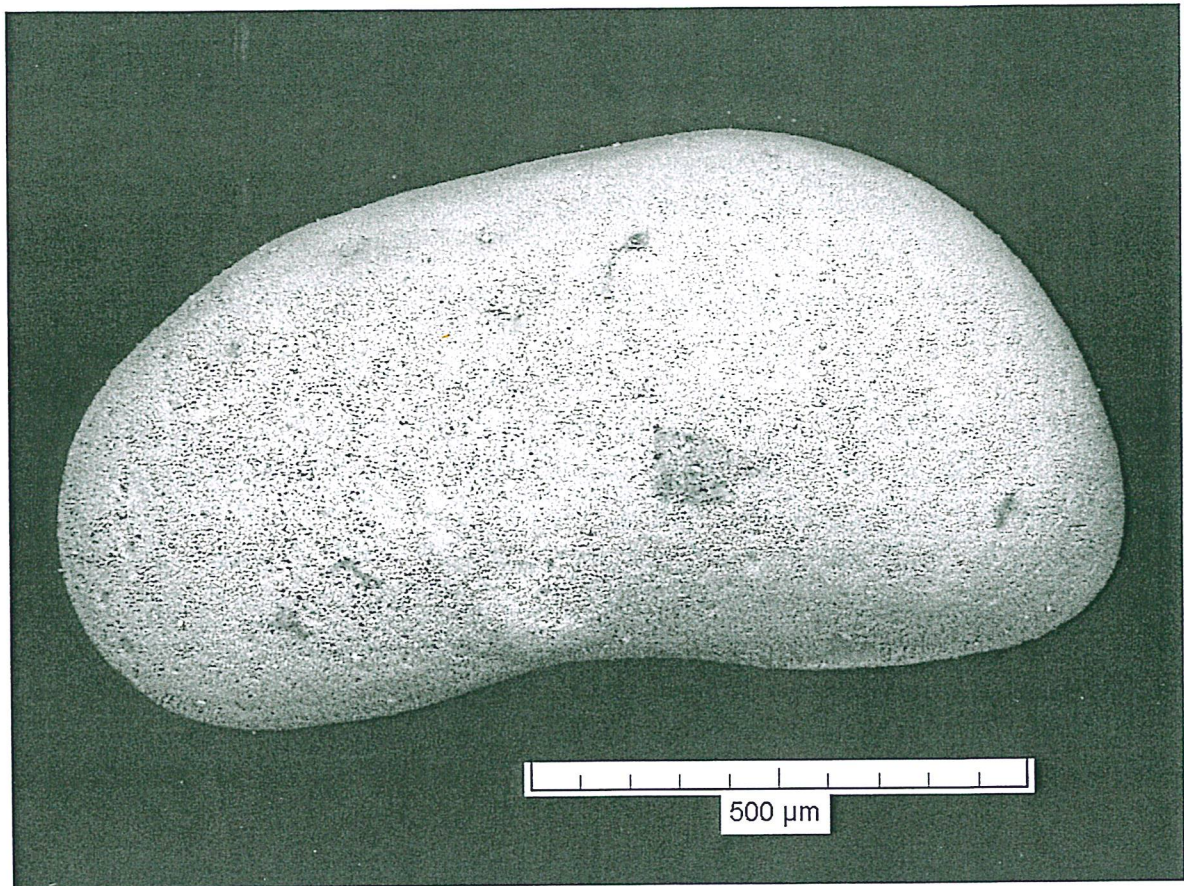
Fig. 4 - Candona neglecta Sars, 1887: left valve, external view.
