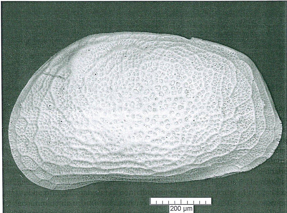
Fig. 3 - Aurila arborescens (Brady, 1865): left valve, external view.
