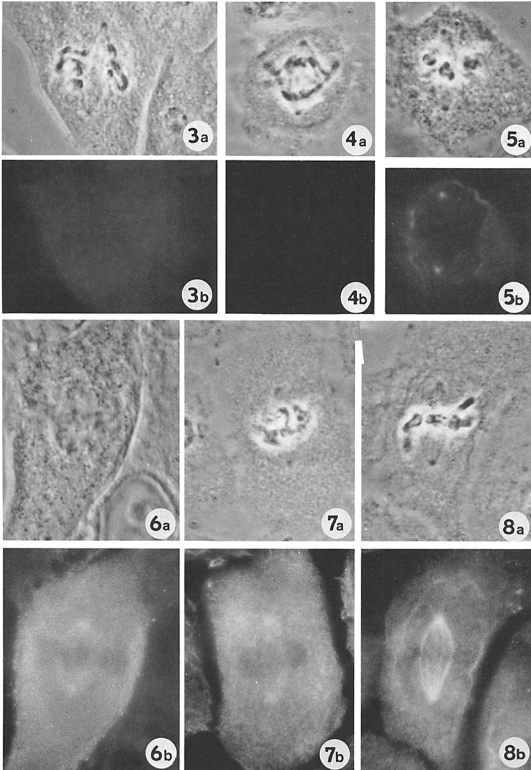
FIGURES 3-4 Indirect immunofluorescence with nonimmune rabbit immunoglobulin. Fig. 3, cell fixed directly in formaldehyde; Fig. 4, cell fixed 7 min after lysis. (a) Phase and (b) fluorescent micrograph of same cell. The magnification of this and all subsequent figures in the paper is \times 2,000 .
