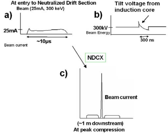
Fig. 1 : A sketch of the longitudinal current compression concept: (a) beam pulse before compression, (b) tilt core voltage waveform applied to uncompressed beam pulse, and (c) compressed beam current.
