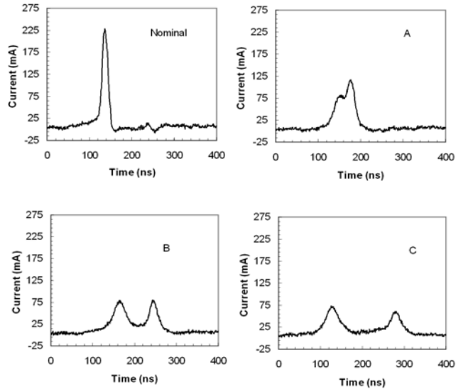
Fig.8: Neutralized drift-compressed beam current with the voltage waveforms in Fig.9.
