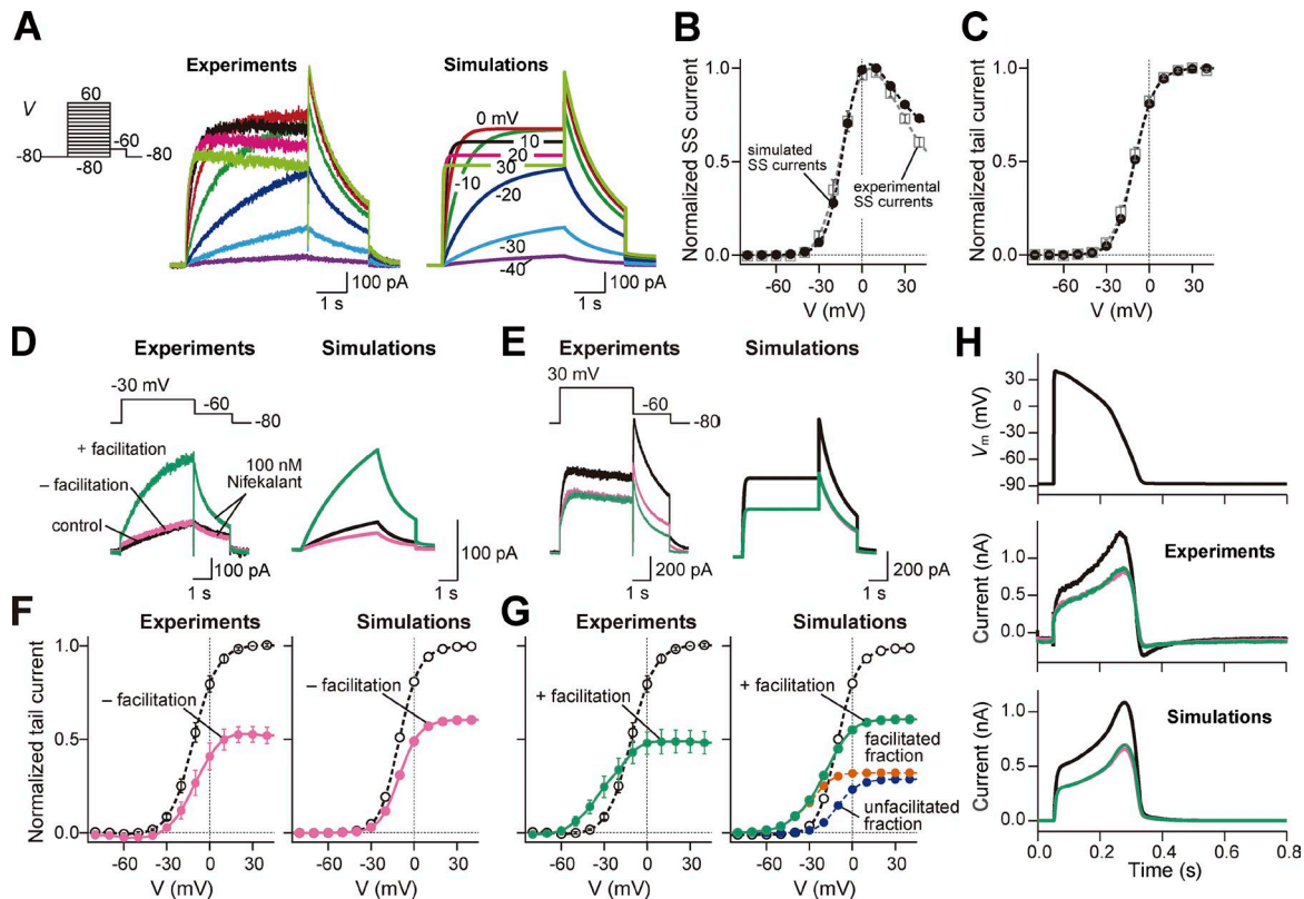
Figure 2. Experimental and simulated macroscopic hERG/ I_{Kr} currents as modified by nifekalant. (A–C) The macroscopic hERG/ I_{Kr} currents in response to voltage-clamp pulses from -80 to +60 mV in 10 -mV increments from a holding potential of -80 mV at room temperature; representative traces (A), the relationship between membrane voltage and the steady-state current amplitude and membrane voltage (B), and the tail current amplitude (activation curve; C). Experimental data are means \pm SEM ( n = 11 ). (D–G) Simulated effects of nifekalant on hERG/ I_{Kr} currents at room temperature condition. The model assumes two populations of channels, with or without facilitation effect by nifekalant ( 100 nM). The V_{1/2} of activation for the facilitated fraction of channel was approximately -31 mV, almost 26 mV negative to that of control channel (see also Materials and methods). (D and E) The macroscopic hERG/ I_{Kr} currents in response to voltage-clamp pulses from -80 to -30 mV (D) or +30 mV (E) at room temperature. (F and G) The relationship between the tail current amplitude and membrane voltage before (F) and after (G) the induction of facilitation effect. Experimental data are means \pm SEM ( n = 5 ). (H) The macroscopic hERG/ I_{Kr} currents in response to cardiac AP at 37^\circ\text{C} . In D–H, black, red, and green solid lines indicate with control, block with facilitation, and conventional block (block without facilitation), respectively. Under the condition in the block with facilitation, I_{Kr} comprises two fractions of I_{Kr} (see also main text), i.e., facilitated and unfacilitated fractions of I_{Kr} . In G right panel, orange and cyan dashed lines represent the facilitated and unfacilitated fractions of I_{Kr} , respectively. Experimental data are means \pm SEM ( n = 6 – 11 ).
