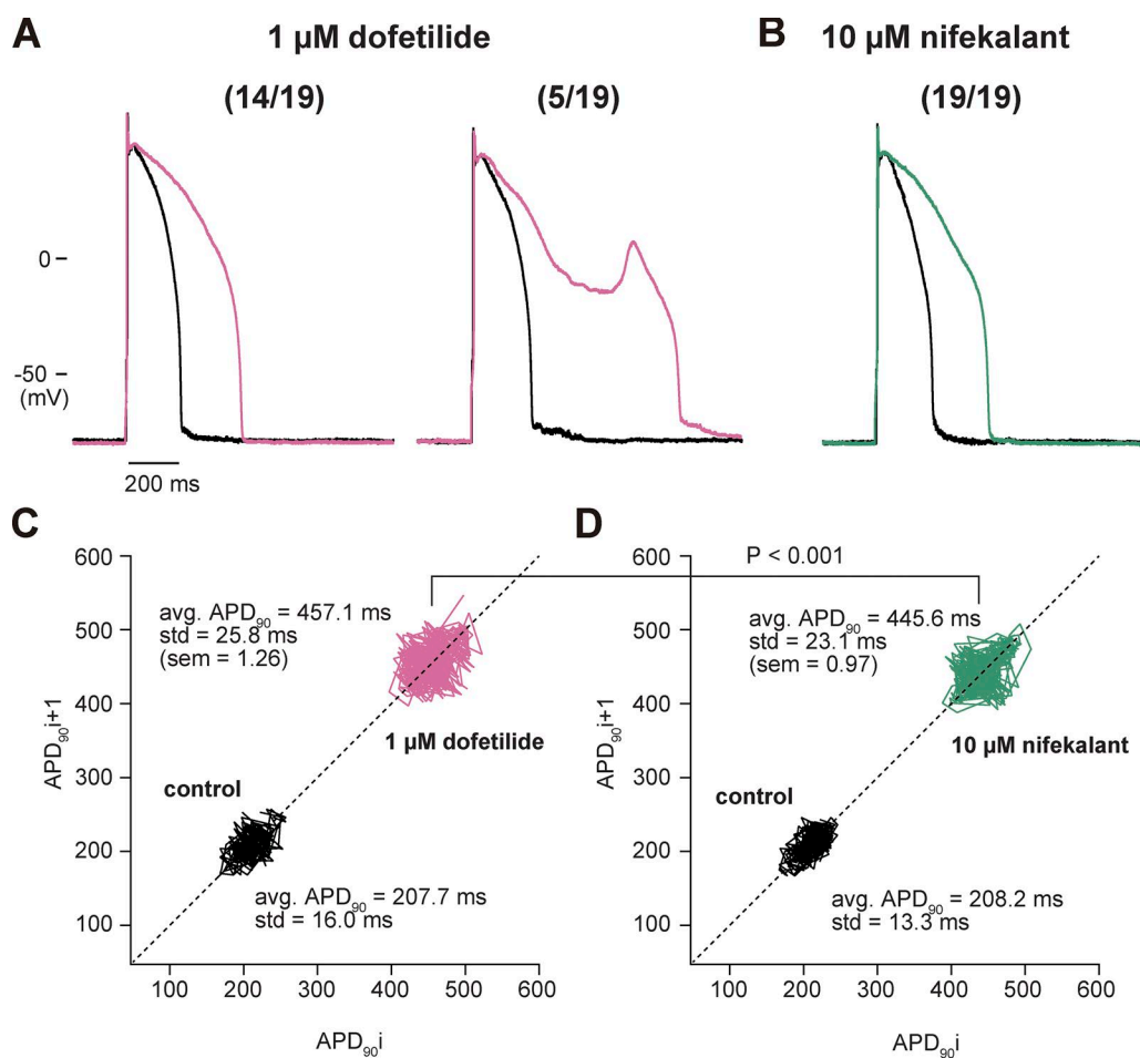
Figure 11. Rabbit cardiac myocyte APs are more stable in nifekalant than dofetilide. AP responses in the isolated rabbit ventricular myocytes were stimulated by minimal current injection at 0.5 Hz in whole-cell current clamp mode at 37°C. (A and B) After recording of the control responses (black lines), cells were treated with either 1 μM dofetilide (pink lines) or 10 μM nifekalant (green line). (A) Representative AP responses without (left) or with (right) EAD in 1 μM dofetilide. Of 19 cells treated with 1 μM dofetilide, five cells showed EAD responses (26%). 14 cells showed the prolongation of APD in 1 μM dofetilide but did not show EAD responses. (B) Representative AP responses in 10 μM nifekalant. All cells treated with 10 μM nifekalant showed prolongation of APD upon 1 μM dofetilide but did not show EAD responses. (C and D) Prolongation of APD and beat-to-beat instability by 1 μM dofetilide and 10 μM nifekalant. Only the data from the cells showing AP responses without EAD were included in this analysis (14 cells of 1 μM dofetilide-treated group; 19 cells of 10 μM nifekalant-treated group). 30 consecutive APs responses in control and under the treatment of either 1 μM dofetilide or 10 μM nifekalant were recorded, and APD 90 of the i +1th action potential (APD 90 i +1 ) was plotted against APD 90 of the one action potential before ( i th; APD 90 i ). APD 90 s were prolonged by treatment with 1 μM dofetilide (C) or 10 μM nifekalant (D) compared with control. 1 μM dofetilide prolonged APD 90 longer (P = 4.26 × 10 -13 , Student's t test) than 10 μM nifekalant. The control APD 90 s were identical between dofetilide- and nifekalant-treated cells (P = 0.58).
