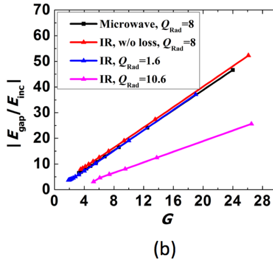
Figure 2.4: The electric field enhancement at the gap (a) as a function of Q , and (b) as a function of G .
