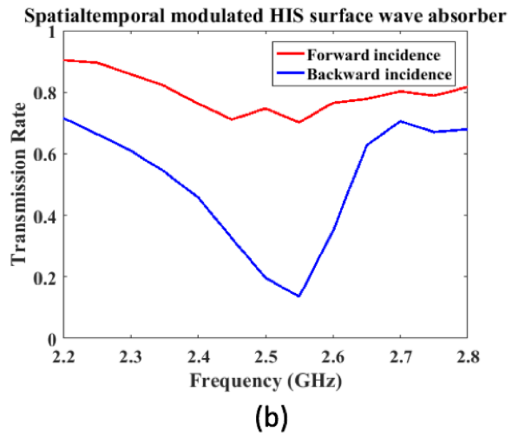
Figure 5.6: EM-circuit co-simulation results. (a) The absorption rate of forward and backward incidence in transient simulation is extracted with via switches modulated in a travelling manner at speed of light with period 1.2ns, 1/3 duty cycle. (b) The transmission rate of forward and backward incidence in transient simulation.
