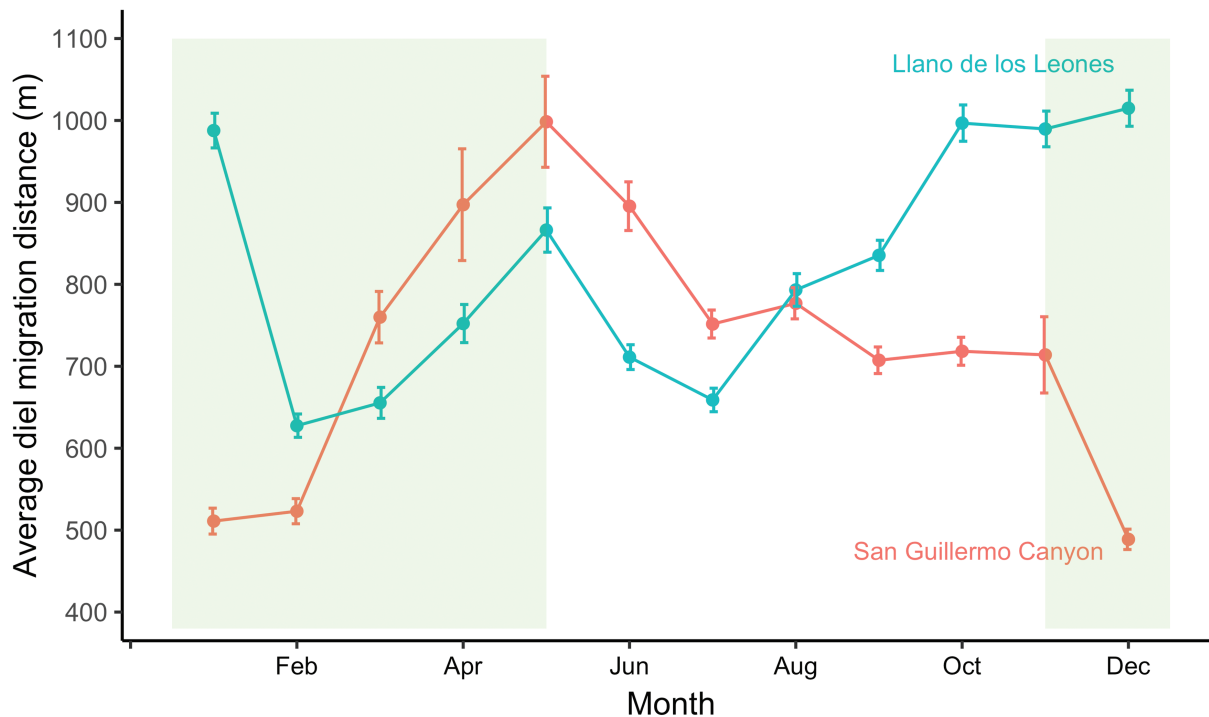
Fig. 2. —A comparison of diel migration distances calculated on a monthly basis for vicuñas in the Llano de los Leones and San Guillermo Canyon for the duration of the study. Diel migration distances increased during the nongrowing period in the Llano de los Leones as compared to the San Guillermo Canyon where distances peak at the beginning of the nongrowing period and subsequently decline. The bars represent 95% confidence intervals based on standard errors. The shaded area represents the growing season.
