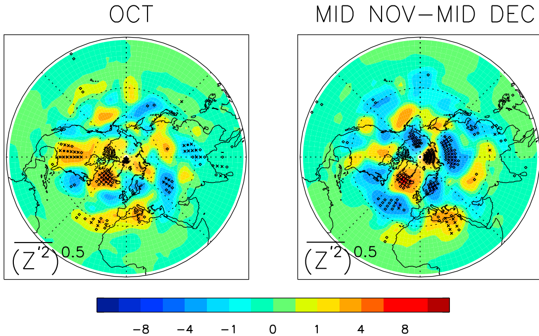
Figure 10. The 500 hPa geopotential height variance (\overline{Z'^2})^{0.5} response for NA snow forcing during (left) October and (right) 15 November to 15 December. Units are meters.
