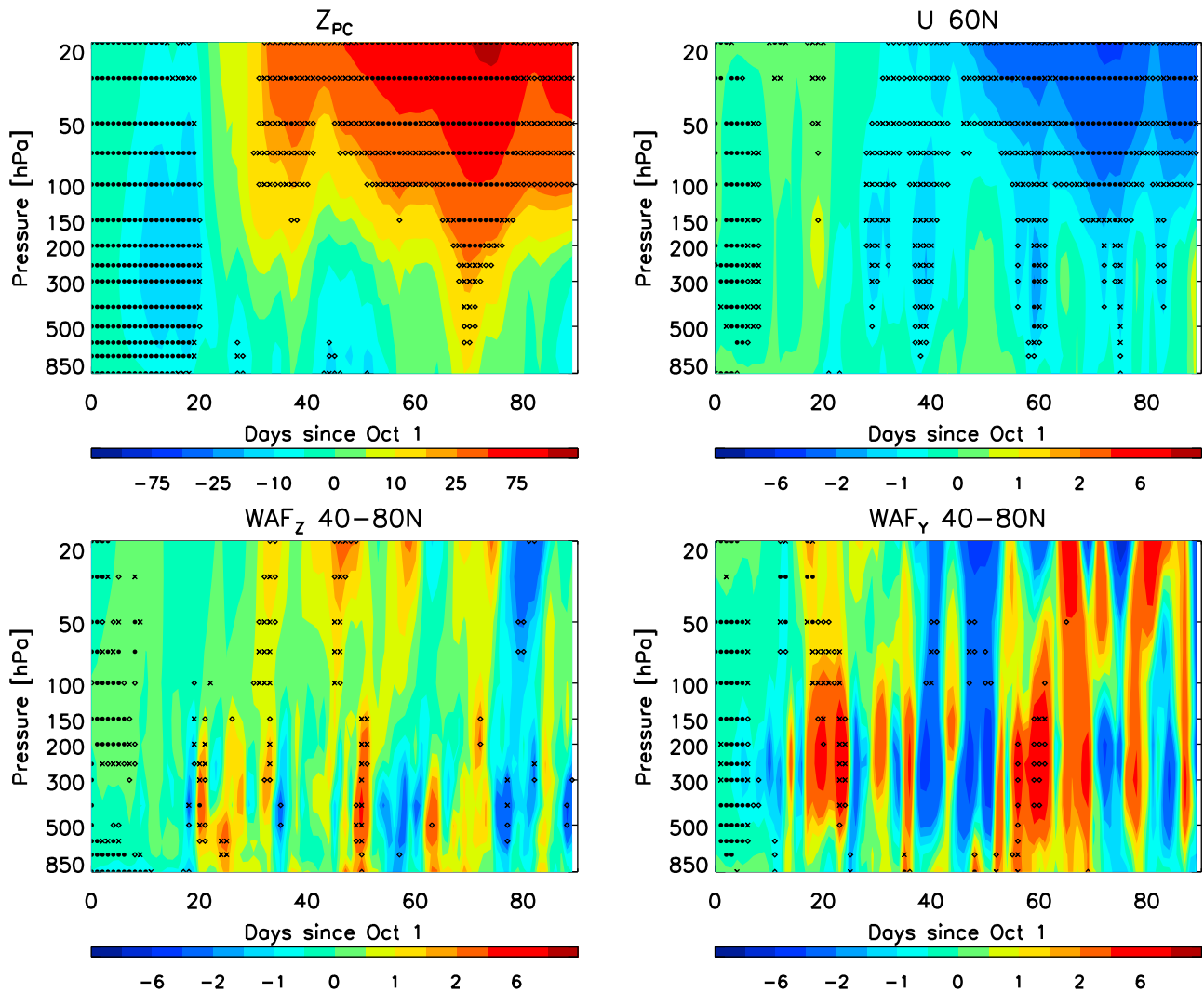
Figure 2. Time-pressure cross sections of the ensemble mean (top left) Z_{PC} , (top right) U 60^{\circ}\text{N} , (bottom left) \text{WAF}_Z 40^{\circ}\text{N} – 80^{\circ}\text{N} , and (bottom right) \text{WAF}_Y 40^{\circ}\text{N} – 80^{\circ}\text{N} response to idealized (climatologically high January) EA snow albedo; units are meters, \text{m s}^{-1} , 10^{-2} \text{m}^2 \text{s}^{-2} , and \text{m}^2 \text{s}^{-2} , respectively. Symbols represent significance as in Figure 1.
