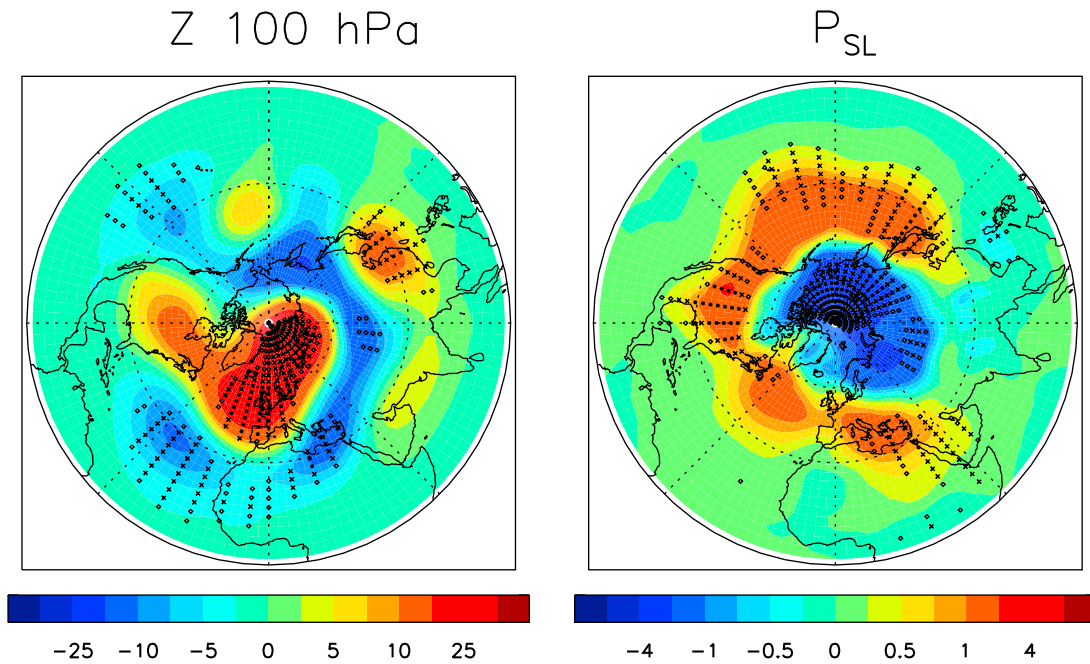
Figure 8. Ensemble mean response to NA snow albedo forcing showing (left) Z 100 hPa for December and (right) P_{SL} for January; units are m and hPa, respectively. Symbols represent significance as in Figure 1.
