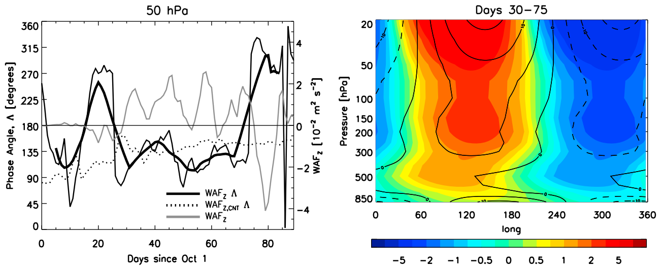
Figure 3. (right) Day 30–75 (i.e., the growth phase) WAF_Z at 60^\circ N for the low-snow control experiment (black lines) and idealized EA response (color shading) for (top) all-waves and (bottom) wavenumber-1. (left) Also included is the time series of the corresponding phase (i.e., longitude of the largest positive WAF_Z ) at 50 hPa and 60^\circ N for the control ( WAF_{Z,CNT} \Delta ; black dashed line) and response ( WAF_Z \Delta ; black solid line), and the WAF_Z response (grey). The thick solid black line represents a 10 day running mean of WAF_Z \Delta . Symbols in the top right panel represent significance as in Figure 1. Units of WAF_Z are 10^{-2} m^2 s^{-2} . Black contour line in right panels has interval of 5 \times 10^{-2} m^2 s^{-2} , with negative values dashed.
