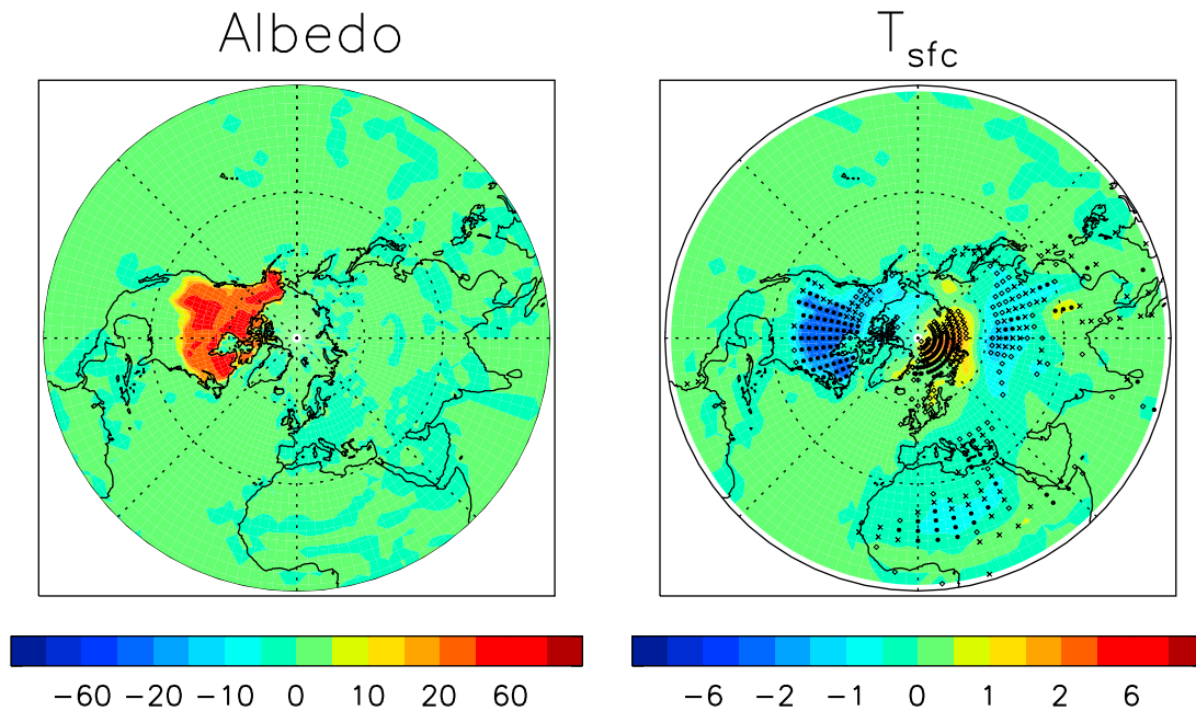
Figure 6. October ensemble mean NA ( 30^{\circ}\text{N} – 90^{\circ}\text{N} and 188^{\circ}\text{E} – 300^{\circ}\text{E} ) (left) snow albedo forcing and (right) December surface temperature response. NA OCT mean \Delta\alpha = 21\% ; \Delta T_{sfc} = -0.73 K. Symbols for \Delta T_{sfc} represent significance as in Figure 1.
