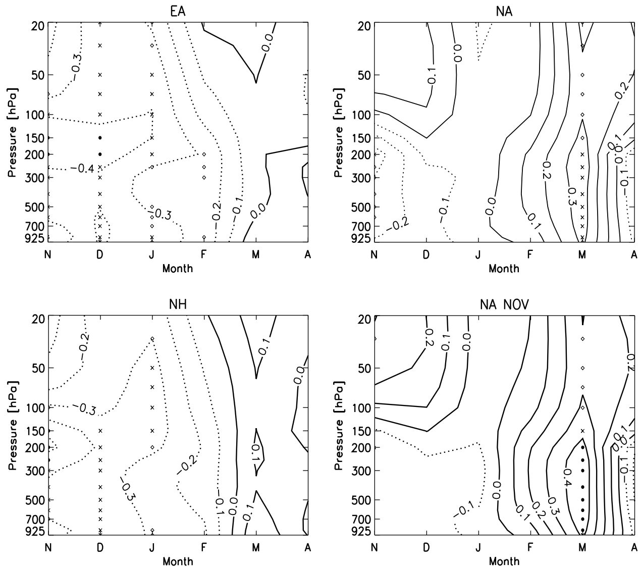
Figure 15. NCEP/NCAR Reanalysis lag correlations between (top left) Eurasian, (top right) North American, and (bottom left) Northern Hemisphere SON snow cover and the AO for November through the subsequent April. (bottom right) Also included is the corresponding North American correlation using November snow. The AO is calculated as the leading principal component of geopotential heights poleward of 20^{\circ}\text{N} , separately for each pressure level. Symbols represent significance as in Figure 1. Negative correlations are dashed lines.
